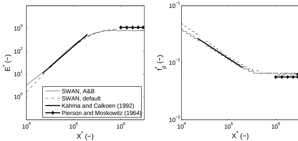
Fig. 1. Deep water, fetch-limited growth curves produced by the source term combination of Eqs. 5 and 8 (A&B), as calibrated, and the default model (Eqs. 3 and 4), both in combination with the DIA. Results for U_{10} = 10 m/s.
