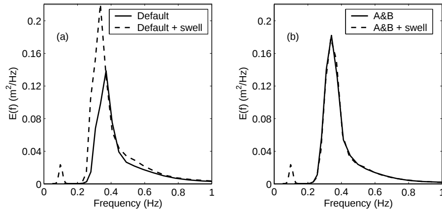
Fig. 4. Influence that background swell has on the wind sea part of the fetch-limited spectra produced by respectively (a) the default source balance and (b) the combination of Eqs. 5 and 8. Results for U_{10} = 10 m/s.
