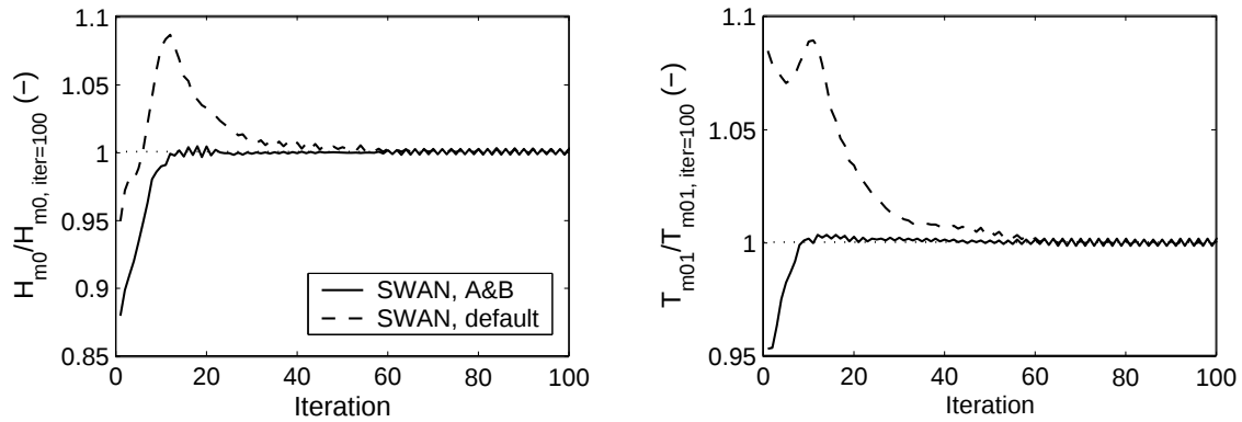
Fig. 5. Comparison of the iteration behaviour of the default model and the combination of Eqs. 5 and 8, for deep water, fetch-limited growth.
