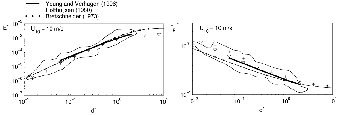
Fig. 2. Depth-limited growth curves produced by the source term combination of Eqs. 5 and 8 (inverted triangles) versus those by the default model (Eqs. 3 and 4, plusses). Observations as indicated. Results for U_{10} = 10 m/s.
