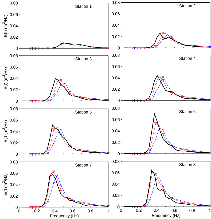
Fig. 3. Lake George observations of near-idealised, depth-limited wave growth. Spectra produced by the source term combination of Eqs. 5 and 8 (inverted triangles) and the default model (plusses). Thick line indicates the observations by the linear array (Stations 1–8) of Young and Verhagen (1996).
