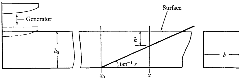
FIGURE 1. Diagram of wave channel showing parabolic wave generator.
