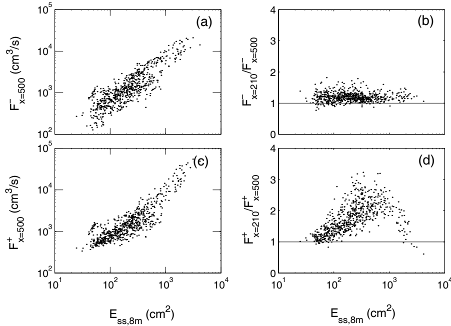
Figure 5. (a) Bulk seaward infragravity energy flux F^- at x = 500 m; (b) bulk ratio of F^- at x = 210 to F^- at x = 500 m; (c) bulk shoreward infragravity energy flux F^+ at x = 500 m; and (d) bulk ratio of F^+ at x = 210 to F^+ at x = 500 m versus sea-swell energy in 8 m depth, E_{ss,8m} .
