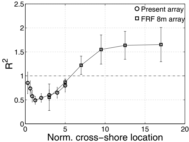
Figure 8. Bulk infragravity reflection coefficient R^2 versus normalized cross-shore location x/x_{50} . Circles are estimates based on collocated p - u sensors ((1), depths less than 6 m) and squares are based on pressure array observations in 8 m depth. The 385 3-hr runs with E_{ss,8m} > 400 \text{ cm}^2 are used.
