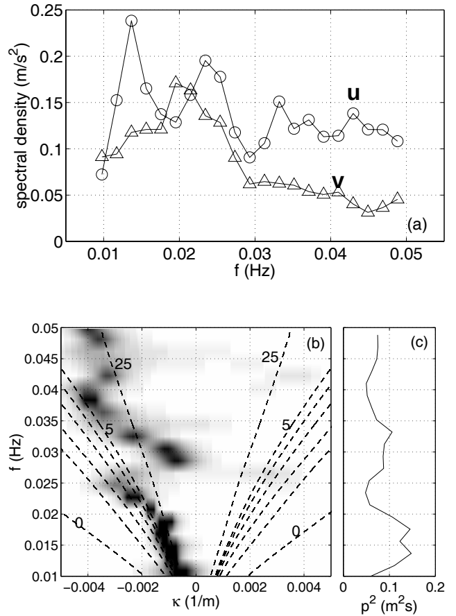
Figure 9. (a) Frequency spectra of infragravity cross-shore u (circles) and alongshore v (triangles) velocities; (b) normalized frequency - cyclic alongshore wavenumber ( f - \kappa ) spectra of pressure p estimated with the Maximum Entropy Method [Wu, 1997]; and (c) frequency spectra of pressure at x = 310 m, on 10 Sept, 0100-0400 hr EST. The dashed curves in (b) are edge wave dispersion curves for modes 0 to 5 and 25 (approximately the boundary between the leaky and trapped wave domains). The f - \kappa spectra at each f are normalized by the frequency spectra, and darker shades indicate higher spectral levels within each frequency band. Additional results for this run are shown in the right-hand panels of Figures 2 and 3.
