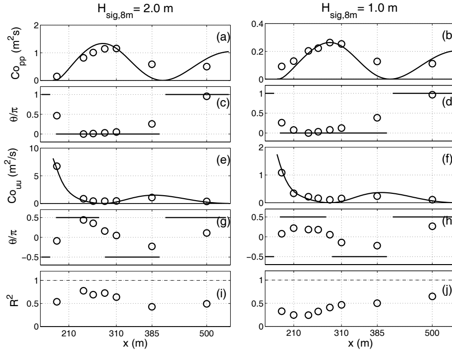
Figure 2. (a,b) Pressure spectral density C_{o_{pp}} ; (c,d) normalized phase difference \theta/\pi between pressure at x = 240 m and pressure at other cross-shore locations; (e,f) cross-shore velocity spectral density C_{o_{uu}} ; (g,h) normalized phase difference \theta/\pi between collocated pressure and cross-shore velocity; and (i,j) infragravity reflection coefficient R^2 versus cross-shore location x . The frequency is 0.014 Hz. In all panels the circles are observations and the solid curves are solutions of the linear shallow water equations for a normally incident cross-shore standing wave ( R^2 = 1 ) on the measured bathymetry. The predicted C_{o_{pp}} and C_{o_{uu}} are normalized with the maximum observed value. Left panels: 7 Nov. 1997, 0700–1000 hr EST, offshore significant sea-swell wave height H_{sig,8m}=2.0 m. Right panels: 10 Sep. 1997, 0100–0400 hr EST, H_{sig,8m}=1.0 m.
