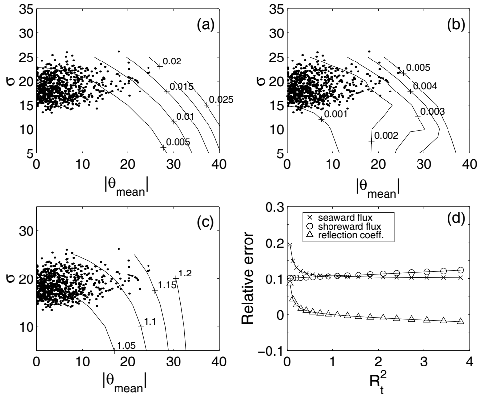
Figure A1. Contours of a) R_0^2 , b) the magnitude of the maximum value attained by |\beta| over a plane beach with a 0.02 slope, over the depth range 1 – 6 m, and c) F_0^+/F_t^+ as functions of the mean direction \theta_m and directional spread \sigma (angular spread function S(\theta) defined in A14). Each dot represents the alongshore-averaged, bulk infragravity mean direction and directional spread for a single 3-hour run at a given cross-shore location, computed with a method that utilizes both components of horizontal velocity [Herbers et al. , 1999]. d) The relative errors of R^2 and F^\pm for R_0^2 = 0.005 , |\beta| = 0.0015 and F_0^+/F_t^+ = 1.1 (eg. the relative error for R^2 is defined as (R^2 - R_t^2)/R_t^2 ) versus the true reflection coefficient R_t^2 .
