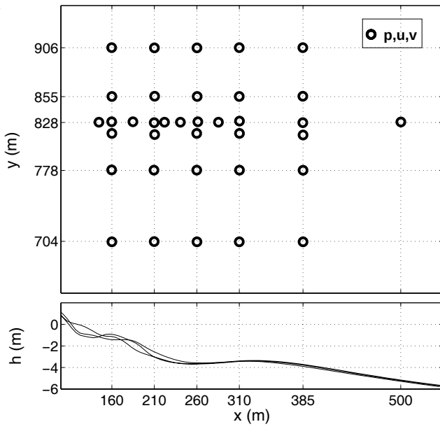
Figure 1. Upper: Plan view of instrument array. Circles are collocated pressure ( p ) and horizontal velocity ( u, v ) sensors. Current meters usually were positioned between 50 and 100 cm above the sea floor. The Field Research Facility coordinate frame is used, with x and y the cross- and alongshore directions, respectively. Additional pressure gauges in 8 m depth ( x = 800 m) are not shown. Lower: Alongshore-averaged sea-floor elevation relative to mean sea level, versus x (collected during August, September, and November).
