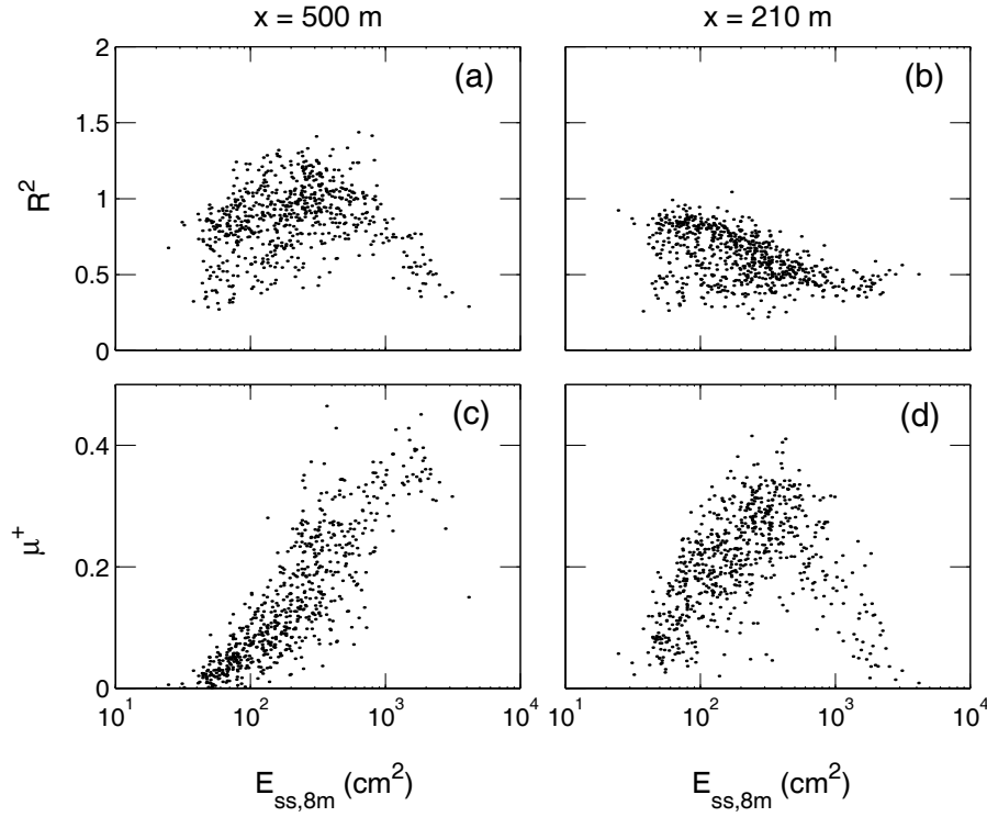
Figure 6. (a,b) Bulk infragravity reflection coefficient R^2 ; and (c,d) bulk nonlinear phase-coupling \mu^+ versus sea-swell energy in 8 m depth E_{ss,8m} , at cross-shore locations x = 500 (left) and 210 m (right).
