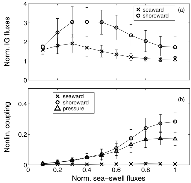
Figure 4. (a) Average values of bulk shoreward F^+ (circles) and seaward F^- (crosses) infragravity energy fluxes normalized by F^-_{x=500} , the seaward infragravity flux at x = 500 m; and (b) bulk nonlinear phase-coupling to sea-swell groups of the total ( \mu , triangles), shoreward propagating ( \mu^+ , circles), and seaward propagating ( \mu^- , crosses) infragravity wave fields versus the shoreward sea-swell energy flux F^+_{ss} normalized by the sea-swell flux in 8 m depth F^+_{ss,8m} . The vertical bars indicate \pm 1 standard deviation about the mean. When offshore sea and swell energy are low, the dominant infragravity waves often are arrivals from remote sources [Herbers et al. , 1995b]. To focus on locally generated infragravity waves, 385 3-hr runs with E_{ss,8m} > 400 \text{ cm}^2 are used.
