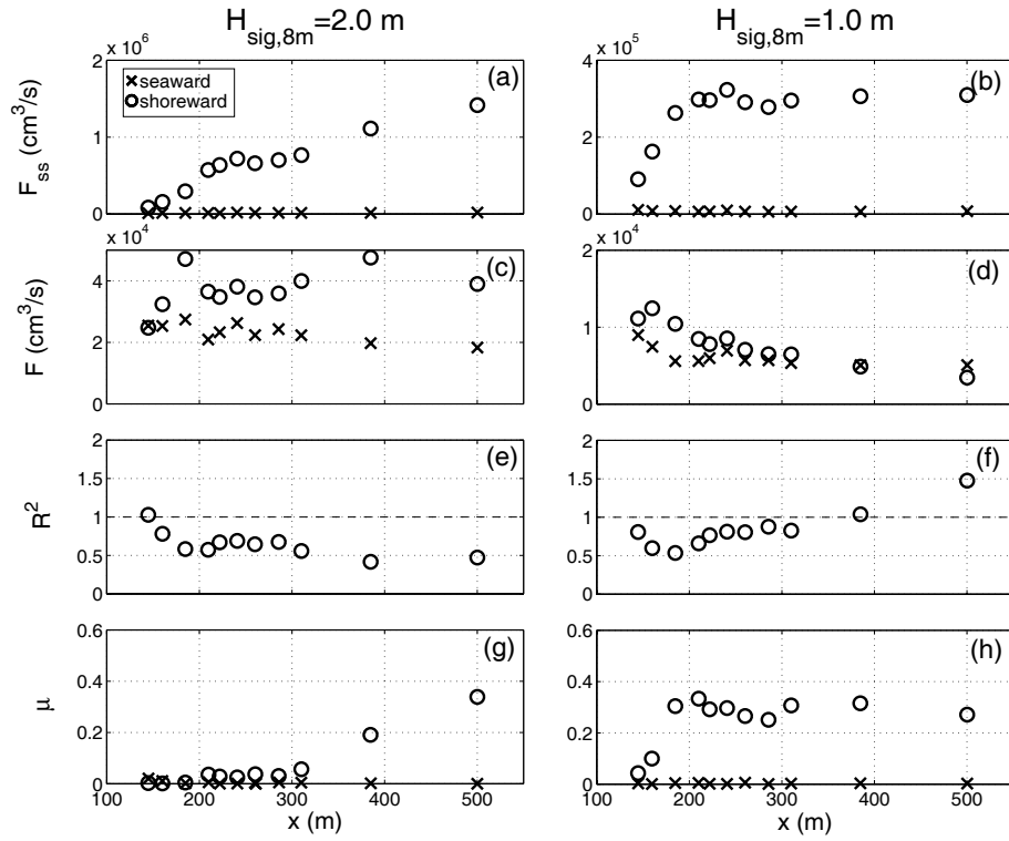
Figure 3. (a,b) Bulk seaward and shoreward sea-swell energy fluxes; (c,d) bulk seaward and shoreward infragravity energy fluxes; (e,f) bulk infragravity reflection coefficient R^2 ; and (g,h) measures of nonlinear phase coupling \mu^+ versus cross-shore location x . The \mu^+ biphases, not shown, are close to 180 degrees, as observed by Ruessink [1998]. Circles and crosses correspond to shoreward and seaward infragravity wave propagation, respectively. Note the different vertical scales for fluxes in the left and right panels. Left panels: 7 Nov 1997, 0700-1000 hr EST, H_{sig,8m}=2.0 m. Right panels: 10 Sep 1997, 0100-0400 hr EST, H_{sig,8m}=1.0 m.
