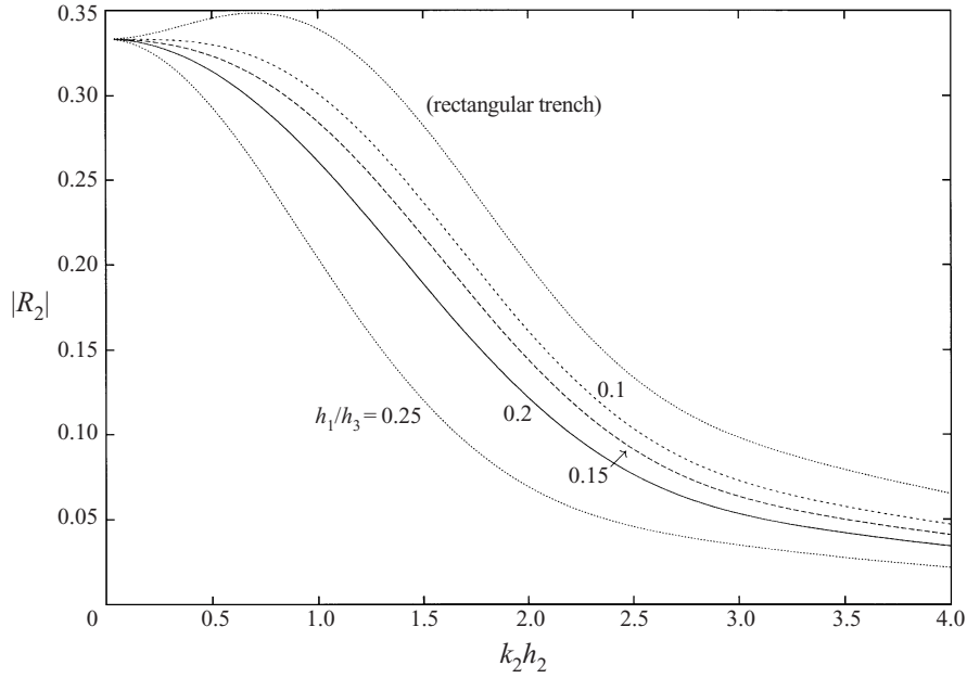
FIGURE 8. Reflection coefficient, |R_2| , against wavenumber k_2 h_2 for the bed profiles \hat{h}(x) defined in (6.6) with h_1/h_2 = \frac{1}{4} , \ell/b = 1 and for different values of h_1/h_3 shown against the curves.
