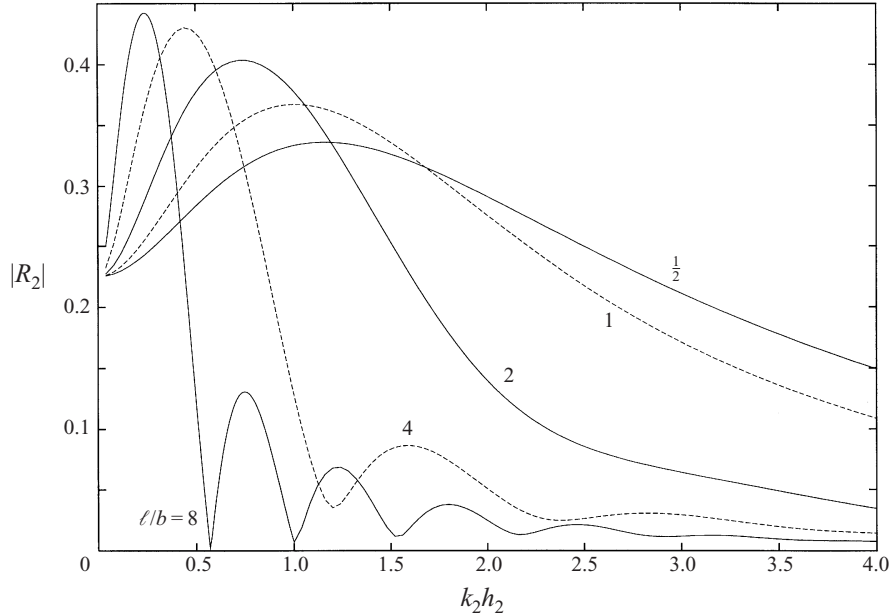
FIGURE 7. Reflection coefficient, |R_2| , against wavenumber k_2 h_2 for the slope profiles given by \hat{h}(x) = 1 - 3x^2 + 2x with h_1/h_2 = \frac{2}{5} , for different values of \ell/b shown against the curves.
