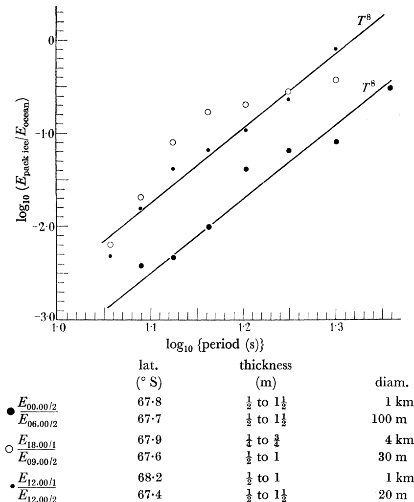
FIGURE 14. Energy penetration into fields of large ice floes as a function of wave period. Return voyage.
