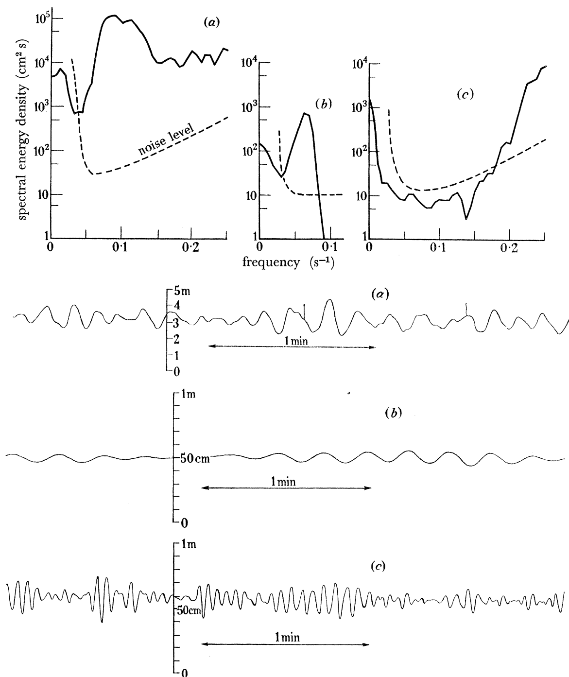
FIGURE 1. Wave records and wave spectra. (a) Open ocean, lat. 55.6° S. Outward voyage. (b) In large ice floes, lat. 69.1° S. Outward voyage. (c) In shore lead, lat. 75.5° S (Halley Bay).
