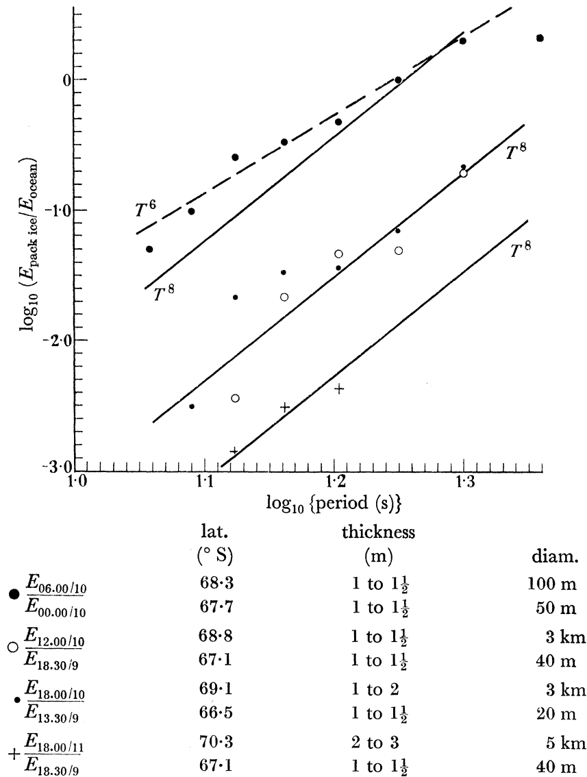
FIGURE 13. Energy penetration into fields of large ice floes as a function of wave period. Outward voyage.
