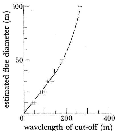
FIGURE 12. Floe diameters and wavelength of cut-off with smaller floes.
