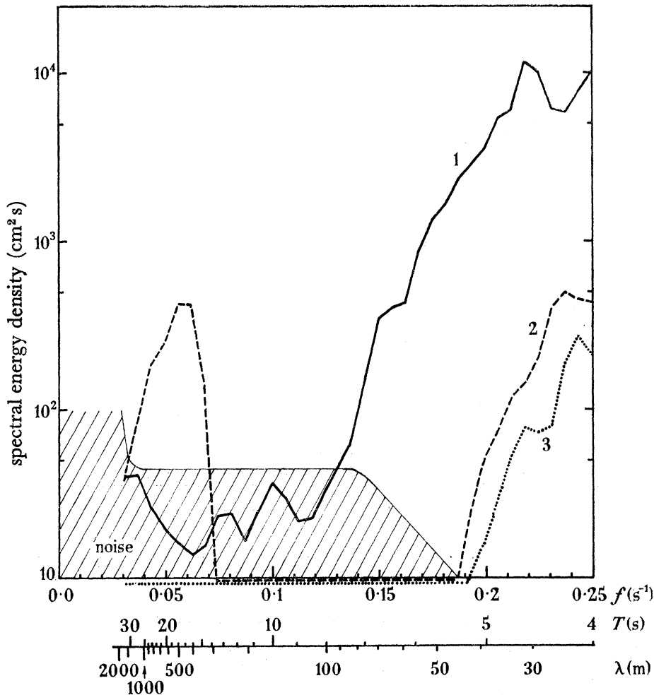
FIGURE 9. Wave spectra in shore lead. 1, 75.5° S, 20 knot wind; 2, 71.1° S, calm; 3, 75.5° S, calm.
