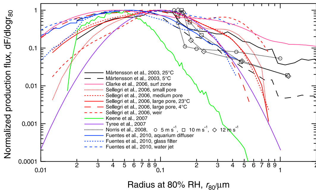
Figure 4. Size distributions of SSA production flux normalized to maximum value in representation dF/d\log r_{80} as a function of r_{80} from laboratory experiments (Mårtensson et al. 's [2003] Figure 4c; Sellegri et al. 's [2006] Figures 2 and 4; Keene et al. 's [2007] Figure 3 for 5 L min -1 ; Tyree et al. 's [2007] Table 1, artificial seawater, and salinity 33; and Fuentes et al. 's [2010] Figure 6) and field measurements (the Clarke et al. [2006] formulation which is presented in text and Norris et al. 's [2008] Figure 6 at U_{10} 5, 10, and 12 m s -1 ). Uncertainties in the original data are not shown.
