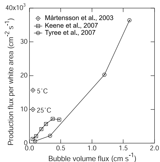
Figure 5. Dependence of total SSA number production flux per white area in laboratory experiments of Mårtensson et al. [2003] using artificial seawater (salinity 33) at two different temperatures, Keene et al. [2007] using natural (low productivity) seawater, and Tyree et al. [2007] using artificial seawater (salinity 33) on bubble volume flux (volume of air in bubbles rising to the water surface per unit area and time).
