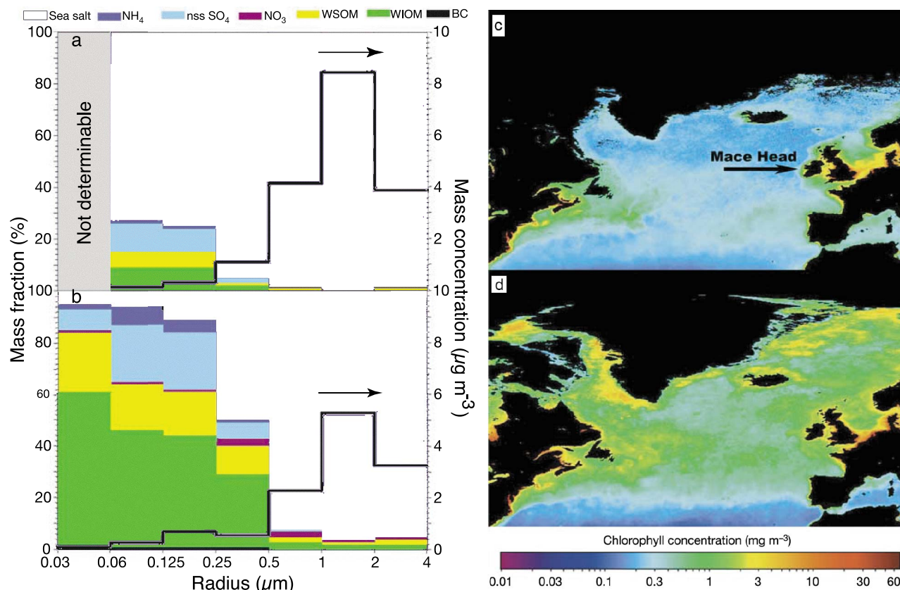
Figure 7. Average mass concentration of total particulate matter (black line, right axis) and mass fraction (colors, left axis) of sea salt, NH 4 , nss SO 4 , NO 3 , WSOM, WIOM, and black carbon (BC) in several size ranges for North Atlantic marine aerosol sampled at Mace Head, Ireland, in clean marine air during periods of (a) low biological activity, November (2002), January (2003), and February (2003) and (b) high biological activity, March–October (2002). Radius corresponds to relative humidity approximately 70%. For low biological activity mass concentrations of aerosol constituents other than sea salt were below detection limits for the size range 0.03–0.06 μm. Oceanic chlorophyll-a concentrations over the North Atlantic for periods of (c) low and (d) high biological activity are 5 year averages (1998–2002) over the same months as for the composition measurements, based on satellite measurements of ocean color (courtesy of Sea-viewing Wide Field-of-view Sensor (SeaWiFS) Project, NASA Goddard Space Flight Center, and Orbital Imaging Corporation (ORBIMAGE)). Adapted from O'Dowd et al. [2004].
