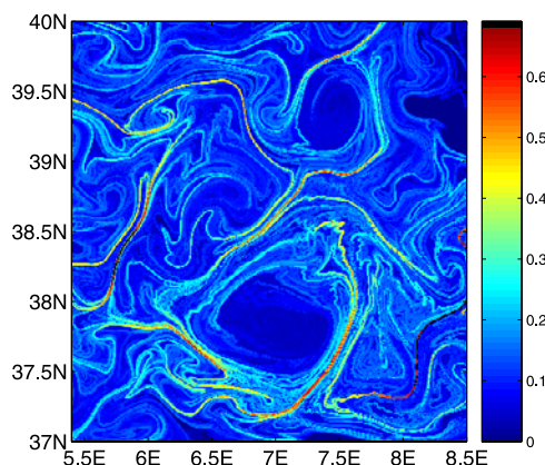
Figure 3. Enlarged plot of the small box shown in Figure 1.
