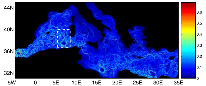
Figure 1. FSLE spatial distribution for the whole Mediterranean on a specific day (10th of June of the first simulation year). \Delta x = \delta_0 = 0.02 degrees. Mesoscale structures and vortices can be clearly seen. Units for FSLEs are \text{day}^{-1} . A zoom of the indicated box is presented in Figure 3.
