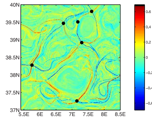
Figure 4. FSLEs calculated from forward (displayed as positive values) and backwards (displayed as negative values) integrations in time, i.e., what is plotted is the field \lambda_+ - \lambda_- . A region with strong mixing appears organized by a tangle of stretching and compressing manifolds. Such lines organize the flow. The black dots indicate some of the hyperbolic points that are located at the intersections of the lines.
