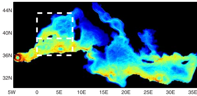
Figure 2. Time average (for the first simulation year) of the FSLEs in the whole Mediterranean basin. Geographical regions of different mixing activity appear. Colors as in Figure 1.
