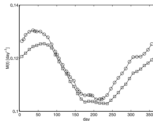
Figure 5. Temporal evolution of the mixing measures M_+(t) (circles), and of M_\pm(t) (squares) for the whole Mediterranean Sea during one simulation year. They display a very similar behavior, with maximum values in winter.
