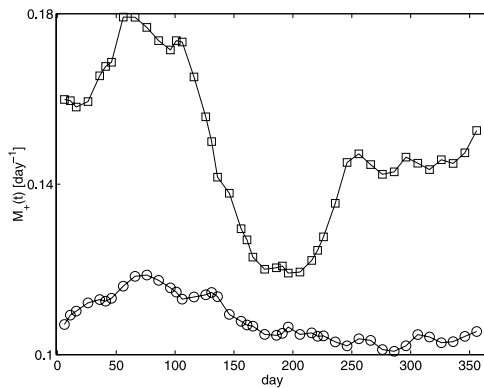
Figure 6. M_+(t) during one year for the Algerian current (squares), which corresponds to the area delimited by the southern box in Figure 2, and the north of the Balearic islands (circles), which is the northern box in Figure 2.
