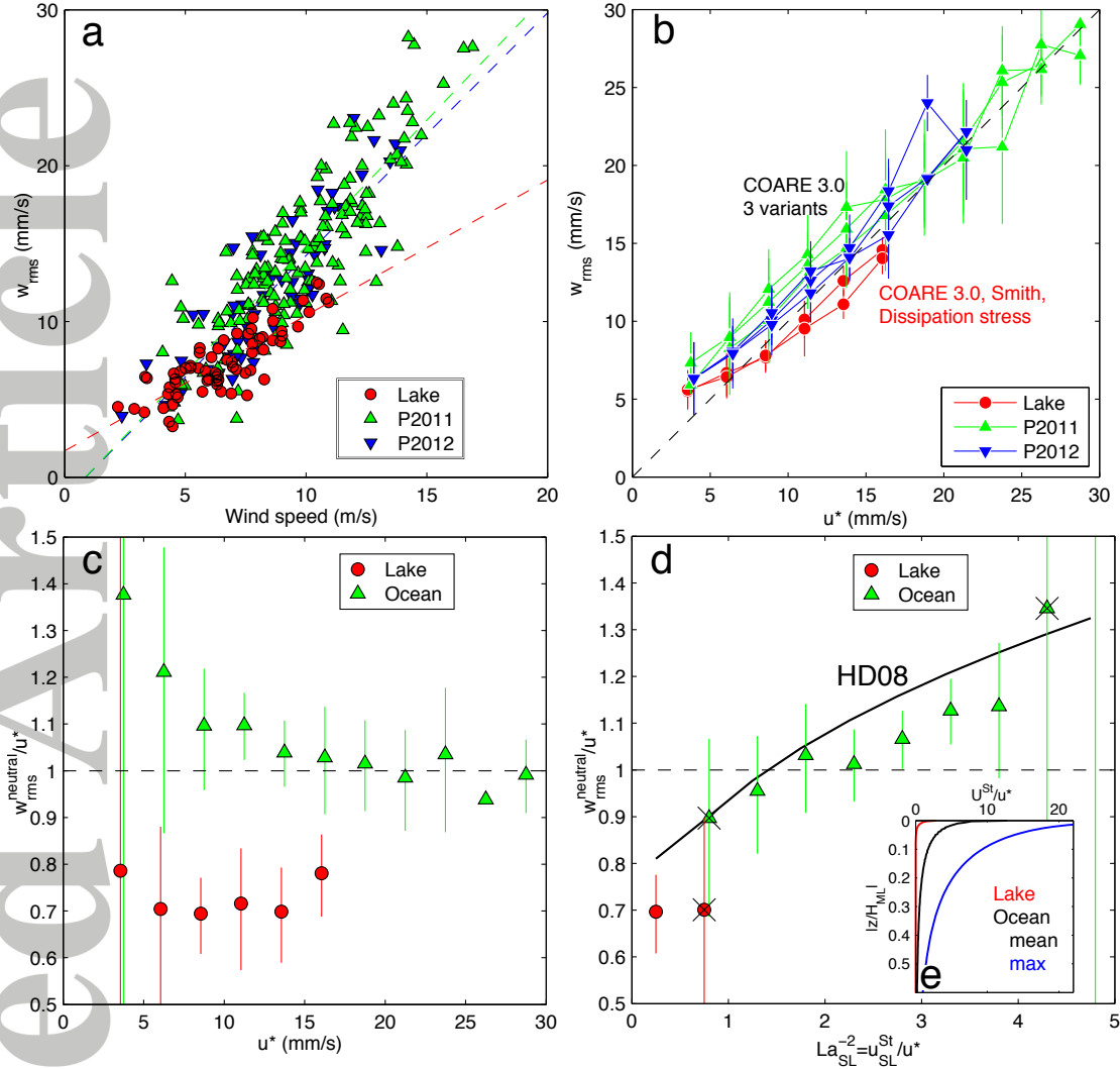
Figure 2. Mixed layer averaged turbulent vertical velocity w_{rms} . a) w_{rms} from different deployments as function of 4m (measured) wind speed. Dashed lines are linear fits. b) w_{rms} from different deployments as a function of u^* . For OWS-P stress computed by three variants of the COARE 3.0 [Fairall et al., 2003] surface roughness are shown (SM 3.5); for the lake stress from COARE 3.0 with the Smith roughness [Smith, 1988] and from dissipation are shown (SM 2.2,2.3). c) w_{rms}^{neutral}/u_* averaged in bins of u_* for lake and ocean data. The COARE 3.0 with the Smith roughness is used. d) w_{rms}^{neutral}/u_* averaged in bins of inverse surface layer Langmuir number La_{SL} squared for lake and ocean data (see Section 3). Heavy line is prediction of Langmuir turbulence [Harcourt and D'Asaro, 2008]. e) Profiles of Stokes drift U^{St} averaged for lake (red), averaged for ocean (black) and the ocean profile with the maximum surface Stokes drift (blue). All confidence limits are 99%. Values of w_{rms} in panels a) and b) are computed from the float pressure (SM 4.2.1) with no additional corrections. Values of w_{rms}^{neutral} in panels c) and d) are corrected for finite float size and buoyancy flux (SM 4.2.3, 4.2.4). In all panels, the lake (red) has a lower value of w_{rms} than does the ocean (green for 2011, blue for 2012) for the same atmospheric forcing.
