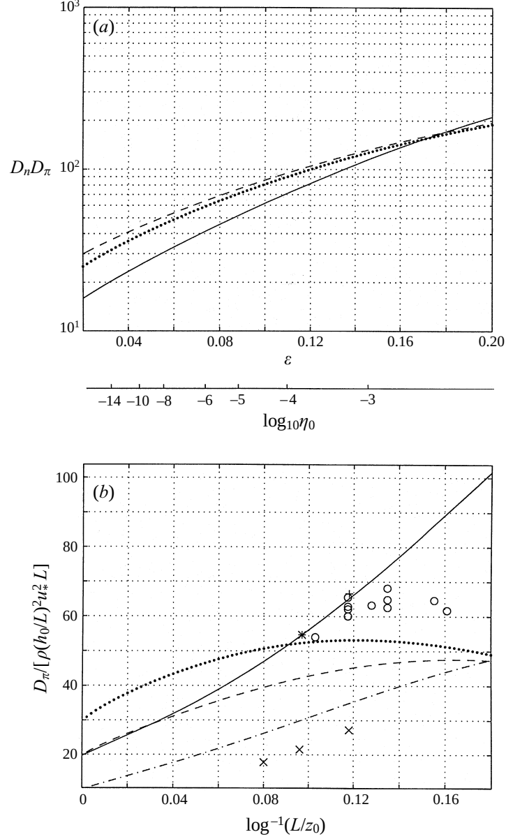
FIGURE 4. (a) The perturbation drag force D_\pi due to pressure and D_n due to nonlinear shear stress as a function of dimensionless roughness length \eta_0 and small parameter \varepsilon for a sinusoidal terrain with wavenumber k = \frac{1}{2}\pi (equations (5.11a) and (5.14a), terms of O(\varepsilon) are omitted in calculation). —, D_\pi for n = 0 ; ---, D_\pi for n = 1 ; \cdots , D_n for n = 1 . (b) Perturbation drag force on a sinusoidal terrain with wavenumber k = \frac{1}{2}\pi : analytical results of present model (5.11a) for \cdots , n = 2 ; ----, n = 1 ; -.-, n = 0 ; —, BNH's truncated mixing-length model; \circ , BNH's numerical computation of second-order closure model; +, Townsend's (1980) numerical model; *, Zilker & Hanratty's (1979) experiment; \times , Townsend's (1972) numerical model.
