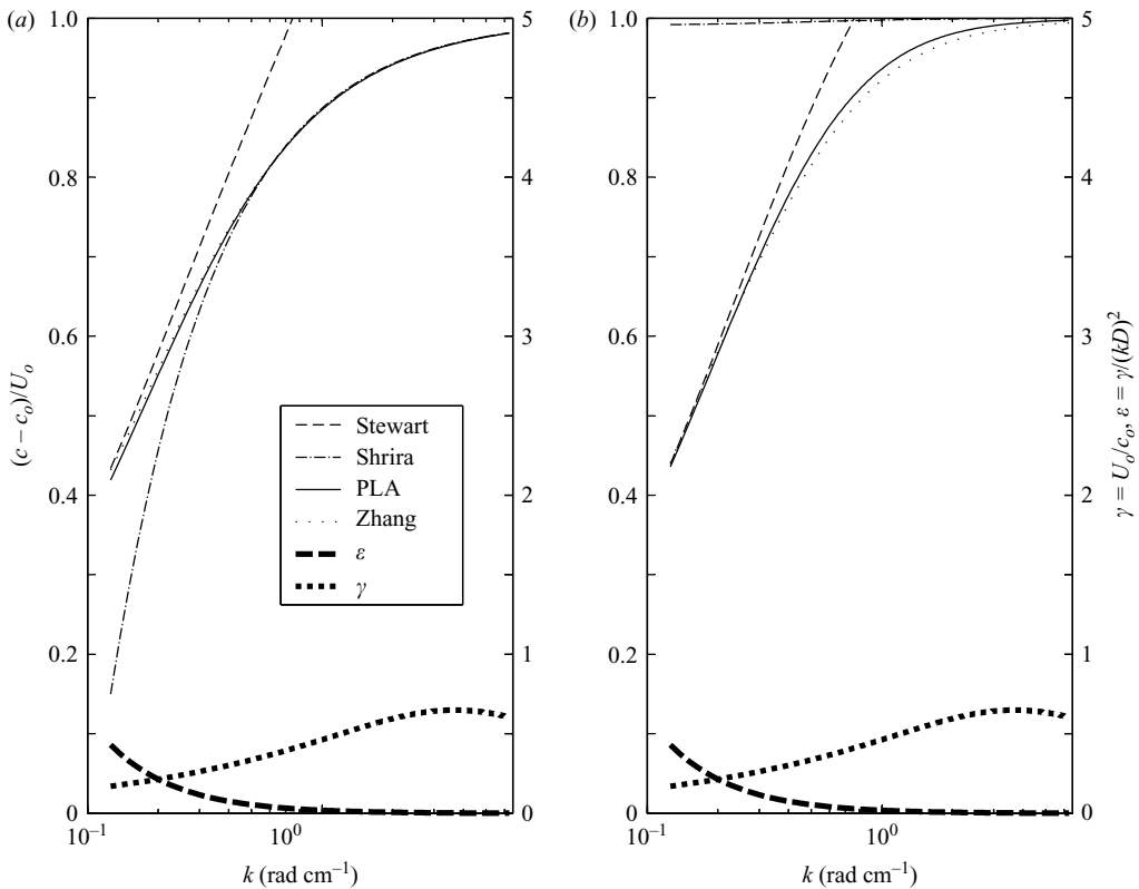
FIGURE 8. Comparison of various approximation schemes. Froude number = 0.21 of weak shear ( D = 5 cm and U_o = 15 cm s ^{-1} ). (a) The Blasius velocity profile Fr = 0.21 and (b) the \text{sech}^2(z) velocity profile, Fr = 0.21 . The thick long and short dashed curves are for non-dimensional scaling constants, \varepsilon and \gamma , respectively, and the scale axis is on the right-hand side. The thin and solid black curve is the calculation using the PLA method, and is used here for reference purposes. The other thin curves represent the different first-order approximations, the dashed thin curves for Stewart & Joy (1974), the dot-dashed curves for Shrira (1993), and the dotted curves for this paper. The surface waves here are in the range of 1 cm to 50 cm.
