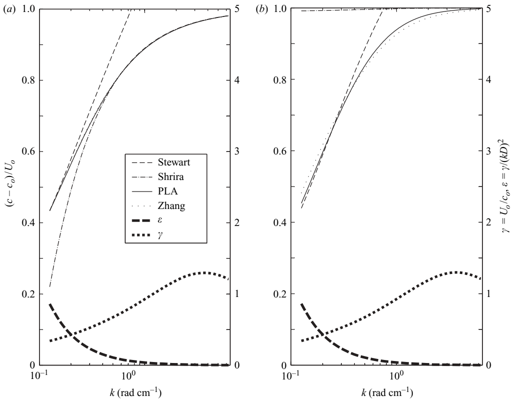
FIGURE 10. Same as figure 8: a comparison of various approximation schemes. Froude number = 0.43 of high wind speed ( D = 4 \text{ cm} and U_o = 30 \text{ cm s}^{-1} ). \gamma becomes large as U_o is comparable to the wave speed in still water for most of the waves, violating the validity condition for Stewart expansion.
