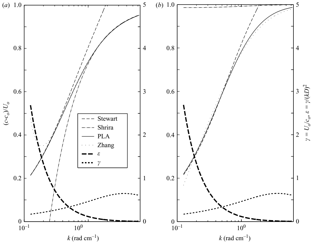
FIGURE 9. Same as figure 8: a comparison of various approximation schemes. Froude number = 0.34 of low wind-speed simulation ( D=2 cm and U_o=15 cm s ^{-1} ). With a smaller shear-layer depth as compared to figure 8, there is less departure from wave speed in still water for longer waves. \epsilon increases quickly towards the long waves, which violates the condition for the Shrira series to converge.
