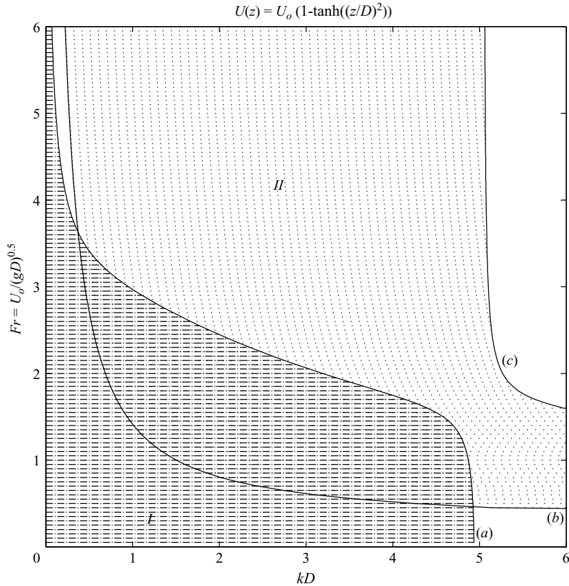
FIGURE 6. Stability diagrams calculated from PLA for the velocity profile \mathcal{U} = \mathcal{U}_o(1 - \tanh(b(y/D)^2)) . No surface tension, i.e. T = 0 . The two shaded regions are the unstable regions, branch I at low wavenumbers and branch II at higher wavenumbers. The curves (a) and (c) are the loci of the neutral solutions associated with the inflection point 0.5218^{1/2} , and the curve (b) is the locus of the neutral solutions with c_s = 0 . There is an overlap region between branches I and II. In the PLA calculations, non-dimensional \Delta z is chosen as 1/20 .
