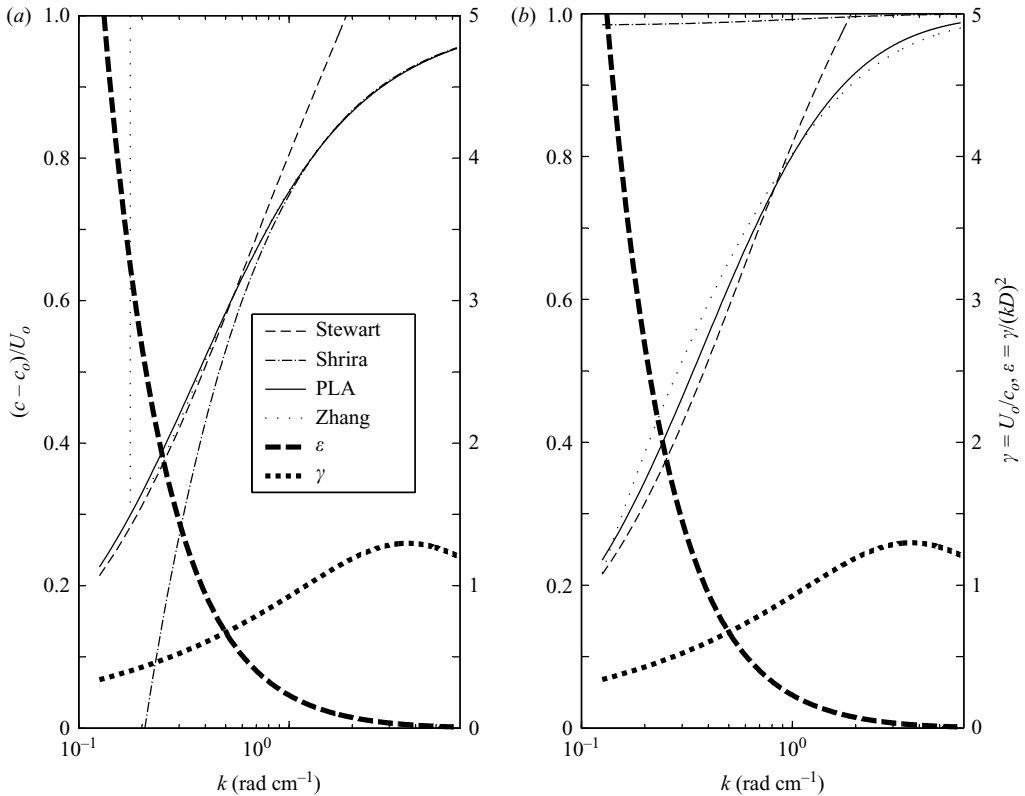
FIGURE 11. Same as figure 8: a comparison of various approximation schemes. Froude number = 0.68 of strong surface shear ( D = 2 cm and U_o = 30 cm s ^{-1} ). For a small shear layer depth, the low wavenumber waves are less affected by the shear. Here both \gamma and \varepsilon are large in the opposite wavenumber ranges.
