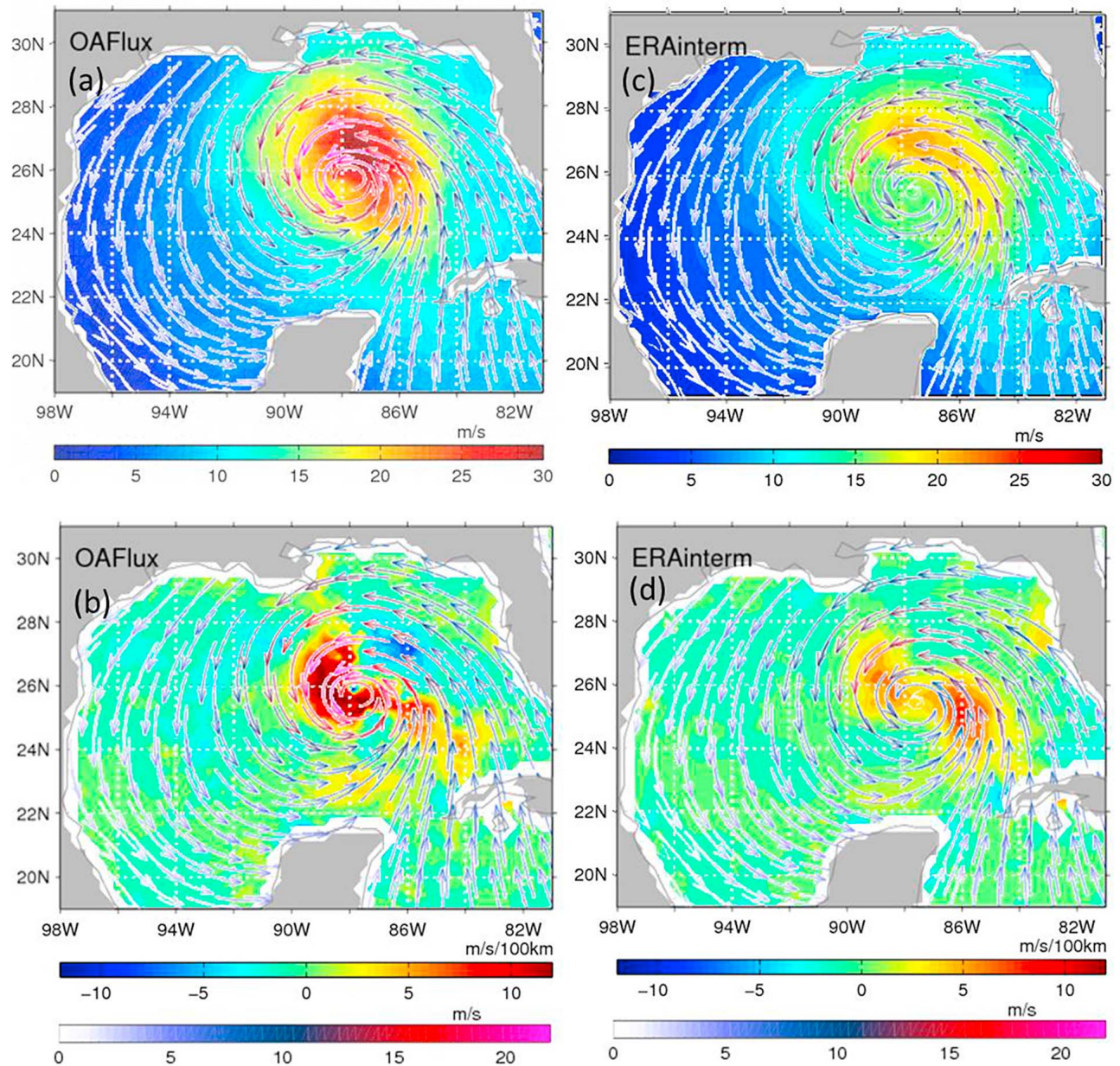
Figure 16. (a) OAFlux daily surface wind speed and (b) wind convergence (positive)/divergence (negative) associated with Hurricane Katrina on 28 August 2005. Surface wind streaklines are superimposed in both plots. (c and d) The same as Figures 16a and 16b but for ERA-interim daily mean that was constructed from averaging six-hourly winds.
