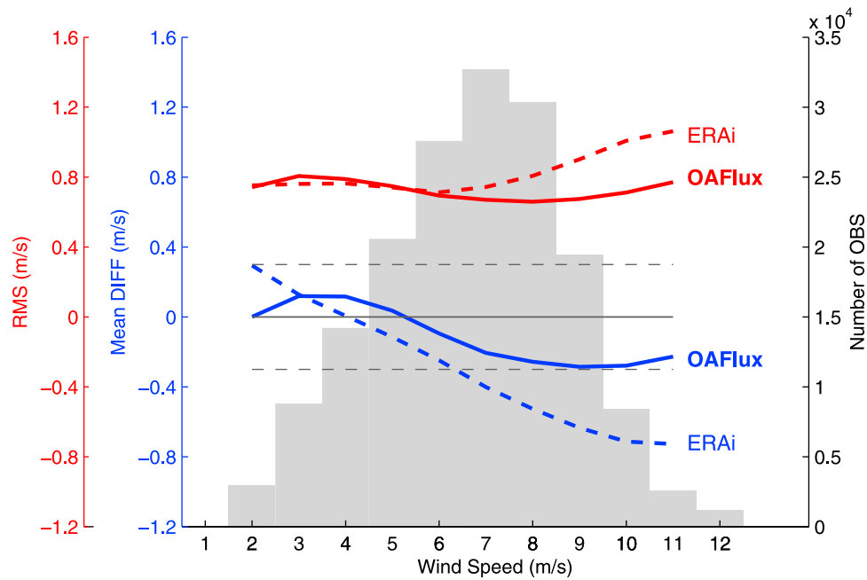
Figure 15. Comparison of mean difference (blue) and RMS difference (red) between daily OAFlux and buoy (solid lines) versus the mean and RMS differences between daily ERAinterim and buoy (dashed lines). The gray dashed line denotes the \pm 0.3 \text{ ms}^{-1} accuracy of buoy wind speed measurements. The background gray bar plot shows the distribution of the number of buoy measurements with wind speed.
