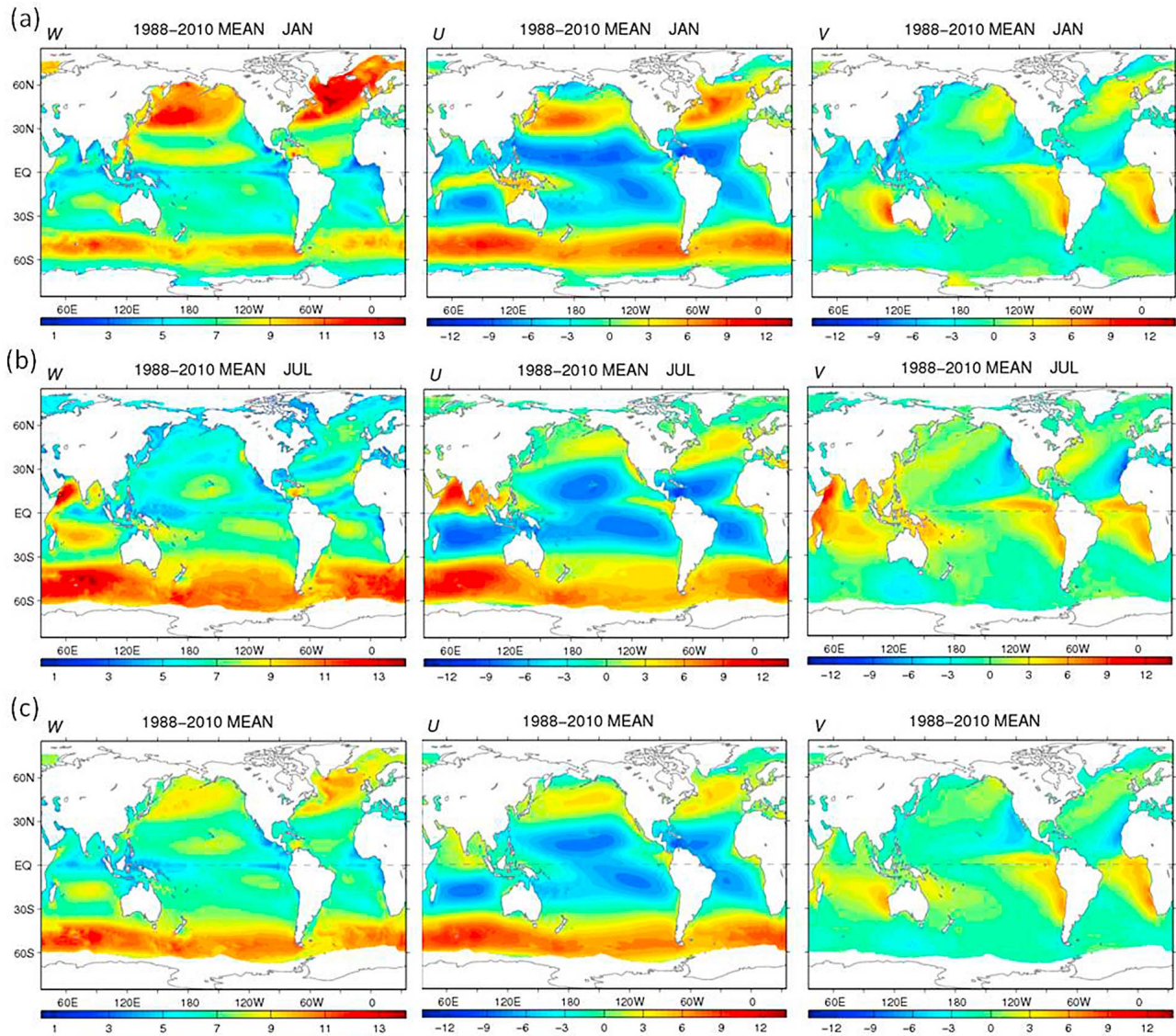
Figure 3. OAFlux mean global fields of near-surface wind speed ( w , left), zonal wind component ( U , middle), and meridional component ( V , right) averaged over the 23 complete years from 1988 to 2010 for (a) January, (b) July, and (c) annual mean.
