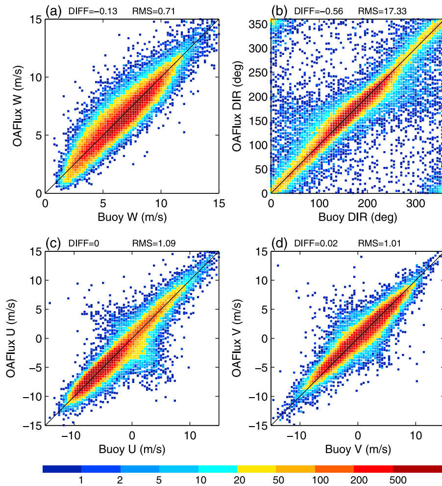
Figure 10. Scatterplots of collocated OAFux and buoy measurements for (a) wind speed, (b) wind direction, (c) zonal wind component, and (d) meridional wind component. There are a total of 168,836 collocations for the period between 1988 and 2010.
