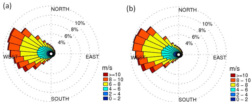
Figure 4. Rose diagram of the percentage of daily wind distribution at all buoy sites from (a) a total of 168,836 buoy daily measurements, and (b) the collocated OAFlux wind analysis. OAFlux has more wind speeds in the range of 0\text{--}8\text{ ms}^{-1} and less wind speeds in the range of 8\text{ ms}^{-1} and higher.
