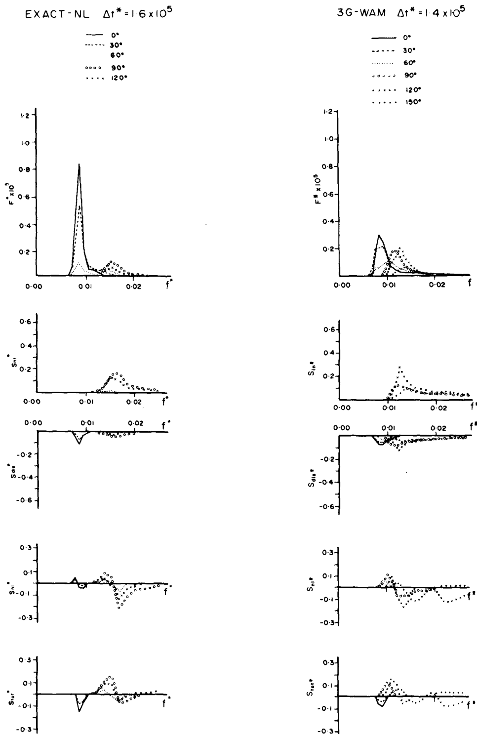
FIG. 6d. As in Fig. 6a but for a wind shift of 120^\circ , \Delta t^* \approx 1.5 \times 10^5 .
