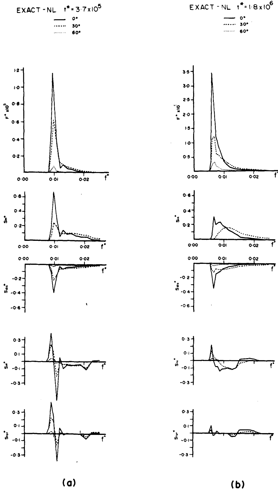
FIG. 4a-b. The source term balance for duration limited growth for the model EXACT-NL: (a) the early stages of growth, t^* = 3.73 \times 10^5 , and (b) the asymptotic stage, t^* = 1.79 \times 10^6 .
