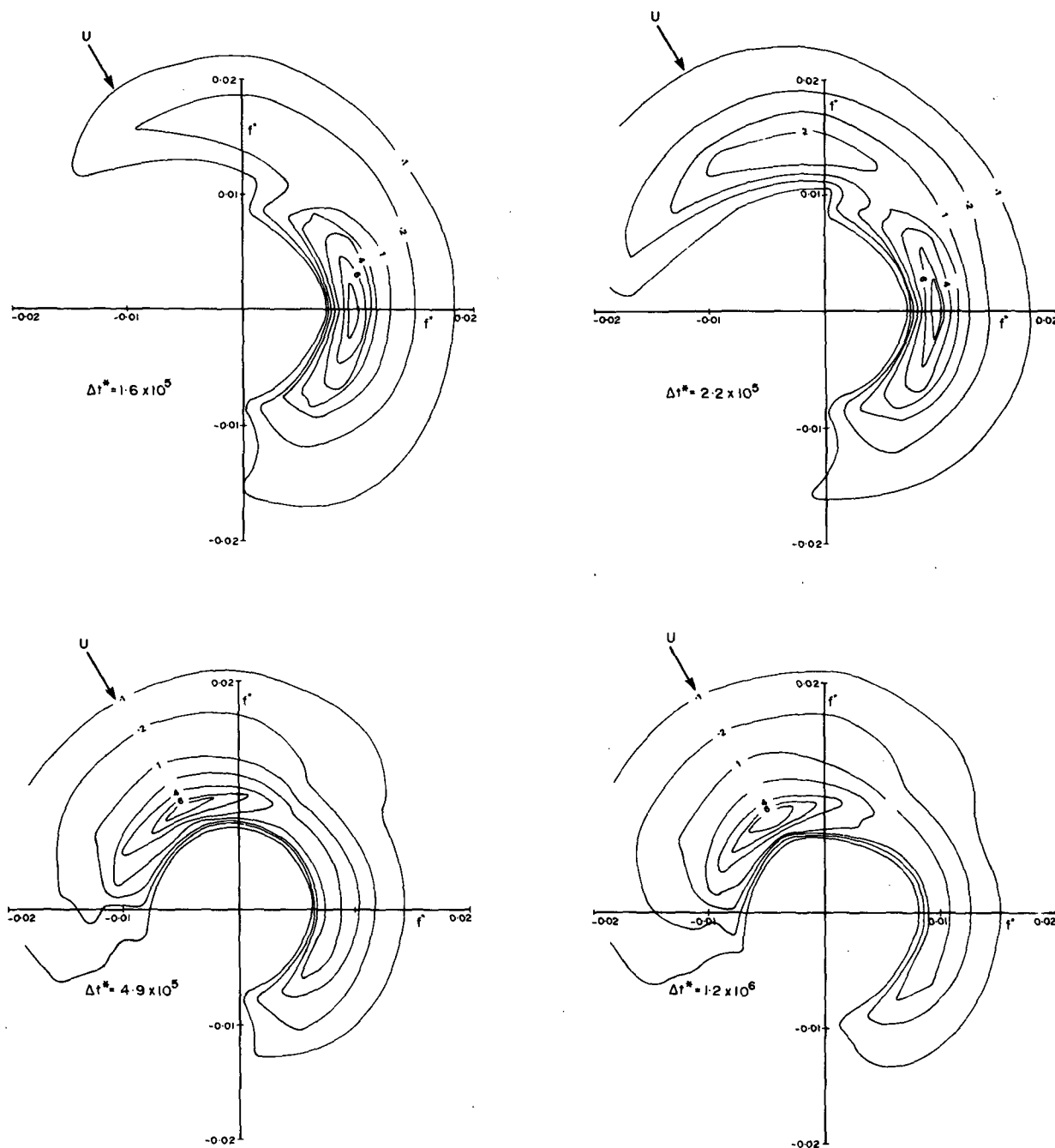
FIG. 5e. (ii) As in Fig. 5e(i) but for the model 3G-WAM.
