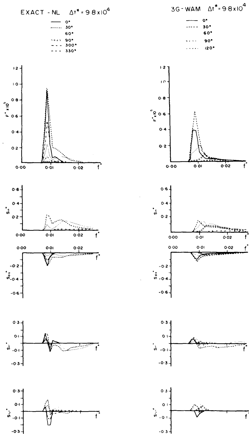
FIG. 6b. As in Fig. 6a but for a wind shift of 60^\circ , \Delta t^* \approx 1.0 \times 10^5 .
