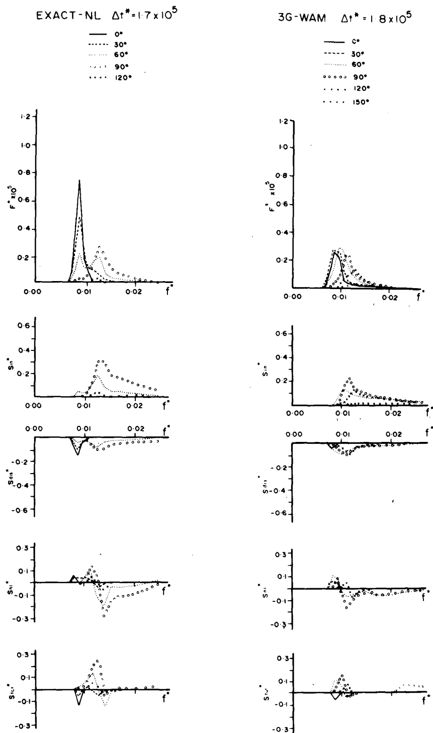
FIG. 6c. As in Fig. 6a but for a wind shift of 90^\circ , \Delta t^* \approx 1.7 \times 10^5 .
