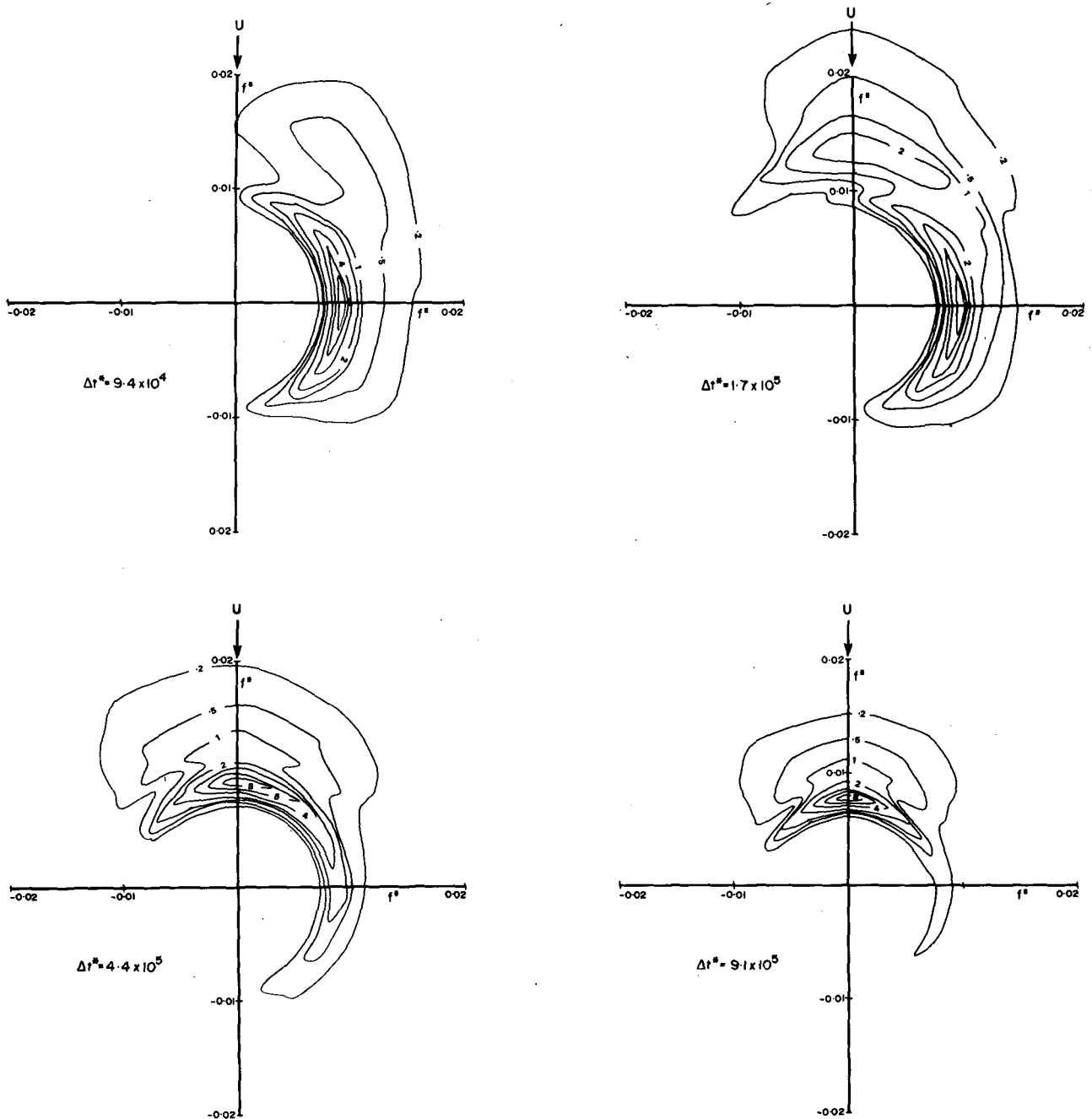
FIG. 5d. (i) Evolution of the directional wave spectrum with time for a wind shift of 90^\circ from model EXACT-NL.
