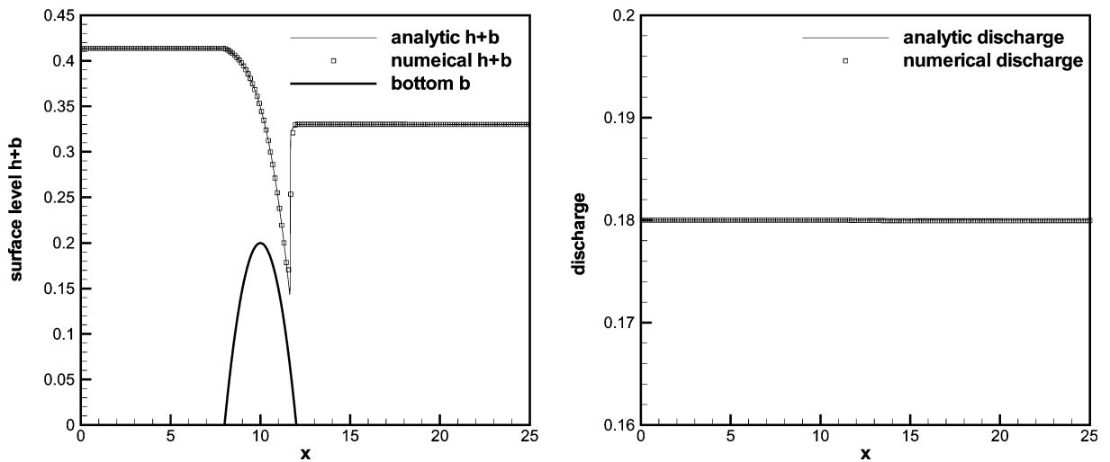
Fig. 12. FV scheme: steady transcritical flow over a bump with a shock. Left: the surface level h+b ; right: the discharge hu as the numerical flux for the water height h .
