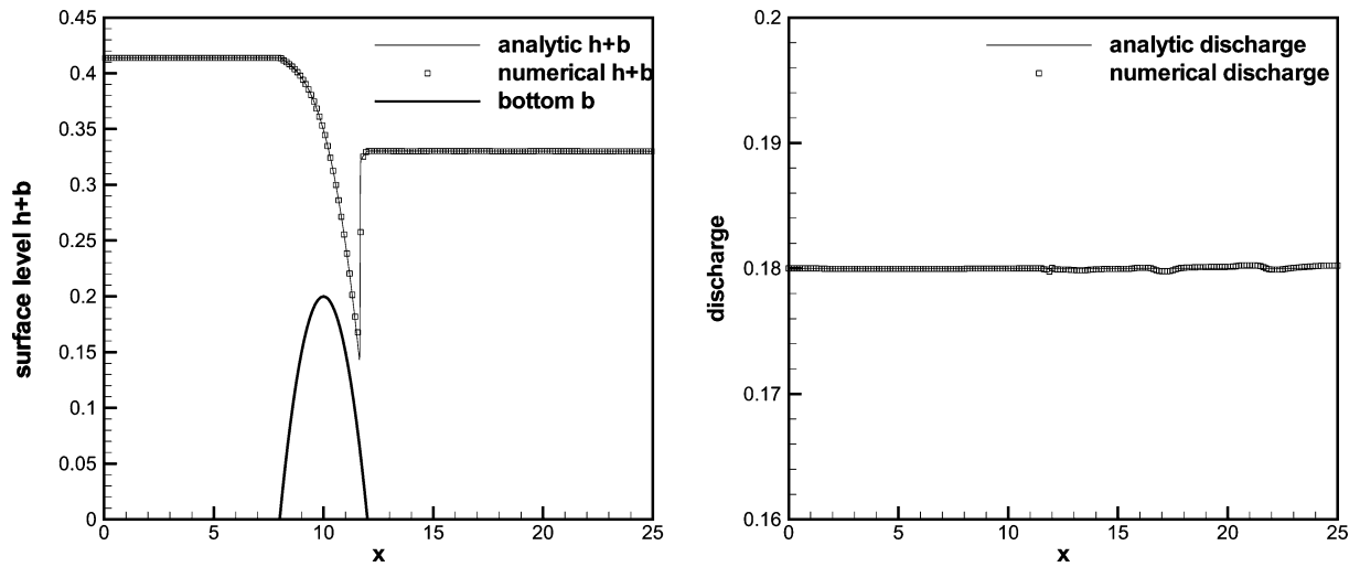
Fig. 14. RKDG scheme: steady transcritical flow over a bump with a shock. Left: the surface level h + b ; right: the discharge hu as the numerical flux for the water height h .
