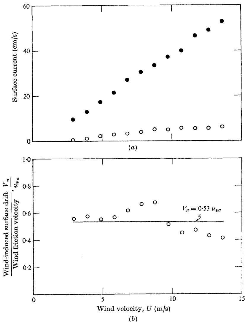
FIGURE 6. Wind-induced and wave-induced surface currents for various wind velocities.
