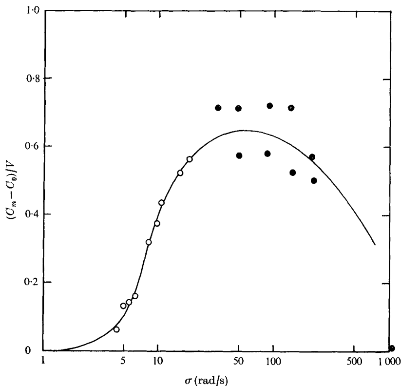
FIGURE 4. Influence of wind drift on wave propagation. \circ , Shemdin (1972); \bullet , Wright & Keller (1971).
