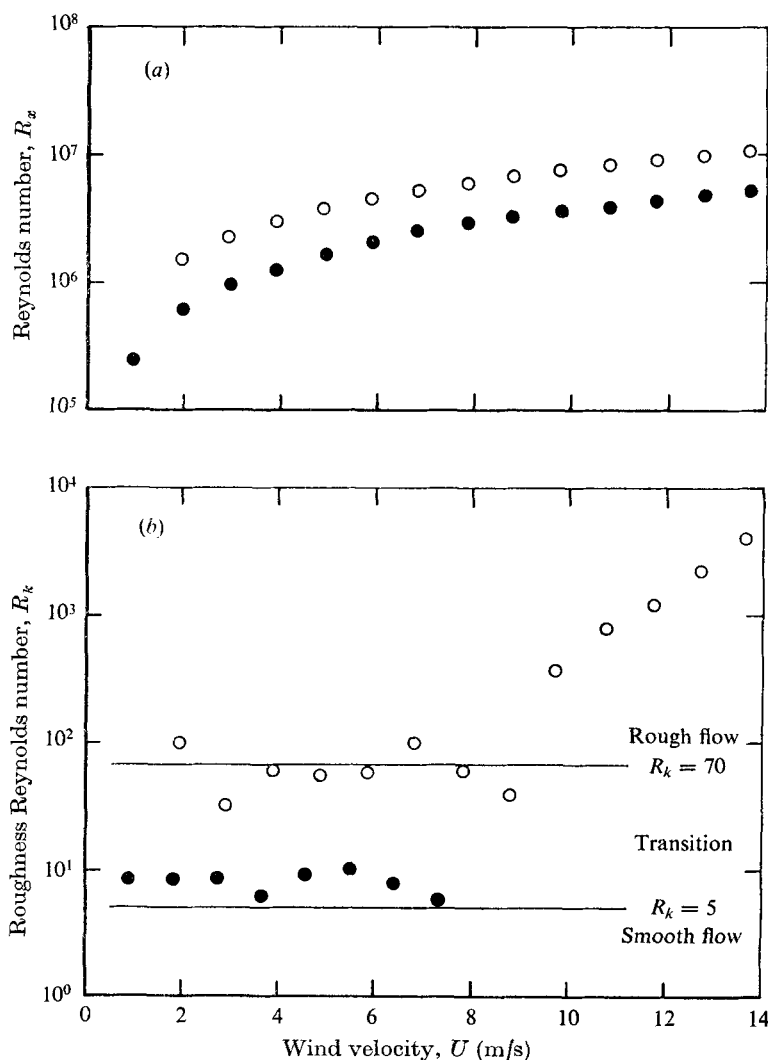
FIGURE 10. Regimes of wind and current boundary layers. \circ , the atmospheric boundary layer; \bullet , aqueous boundary layer. The data used here for the aqueous boundary layer are those obtained with floats.
