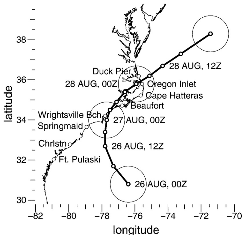
FIG. 1. NHC best-track eye locations for Hurricane Bonnie (thick circles) in 1998. Thin circles indicate tide gauge locations at Duck Pier ( 36.18^{\circ}\text{N} , 75.75^{\circ}\text{W} ), Oregon Inlet ( 35.79^{\circ}\text{N} , 75.55^{\circ}\text{W} ), Cape Hatteras ( 35.22^{\circ}\text{N} , 75.63^{\circ}\text{W} ), Beaufort ( 34.72^{\circ}\text{N} , 76.76^{\circ}\text{W} ), in North Carolina; Springmaid Pier ( 33.65^{\circ}\text{N} , 78.92^{\circ}\text{W} ) and Charleston ( 32.78^{\circ}\text{N} , 79.92^{\circ}\text{W} ) in South Carolina; and Fort Pulaski ( 32.03^{\circ}\text{N} , 80.90^{\circ}\text{W} ) in Georgia. The tide gauge at Wrightsville Beach ( 34.21^{\circ}\text{N} , 77.79^{\circ}\text{W} ) was not placed in operation until 2004.
