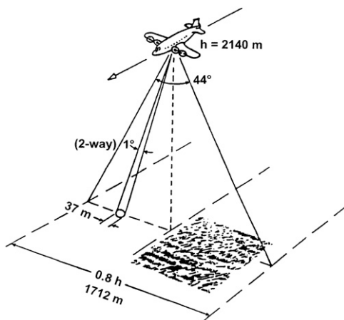
FIG. 4. SRA measurement geometry.
