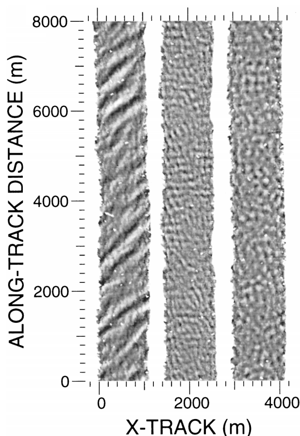
FIG. 3. Wave topography maps produced by the SRA displayed with the same grayscale coding (dark troughs and light crests). The isolated white speckles and the white line at 3700 m along-track and 200 m cross-track are data dropouts. The left-hand and middle images involve about 550 cross-track scan lines acquired over 71 s. The right-hand image involves only about 400 scan lines acquired over 51 s because the aircraft ground speed was faster.
