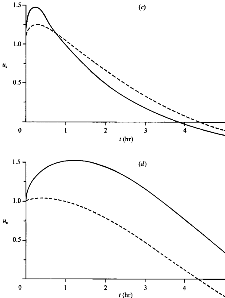
FIGURE 1. Dimensionless surface velocity component u_s = u(c = 0) from (4.15) (solid line) and (4.16) (broken line) versus time. Here \nu_1 = 0.14 \text{ cm}^2 \text{ s}^{-1} and \nu_2 = 0.012 \text{ cm}^2 \text{ s}^{-1} . (a) \lambda = 1 \text{ cm} , (b) \lambda = 10 \text{ cm} , (c) \lambda = 10^3 \text{ cm} , (d) \lambda = 10^3 \text{ cm} . (The dimensional velocity scale here is \zeta_0^2 \omega k ; see the text for meaning of symbols.)
