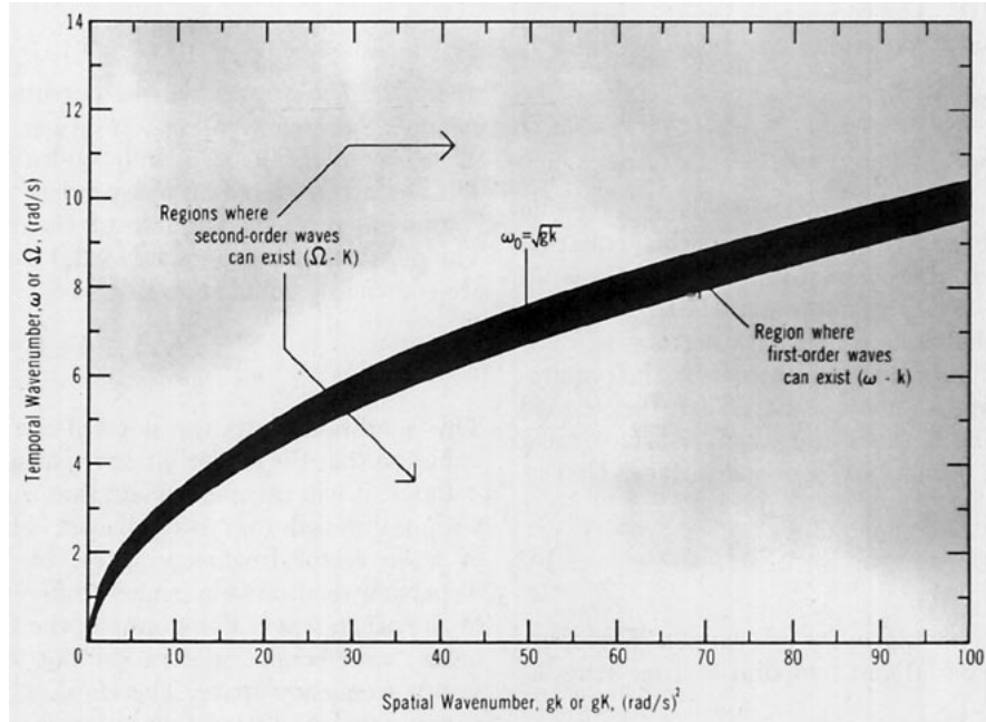
FIG. 1. Gravity-wave dispersion relationship diagram. First-order waves exist in heavily shaded region on \omega_0 = \sqrt{gk} . Second-order waves exist in remainder of diagram.
