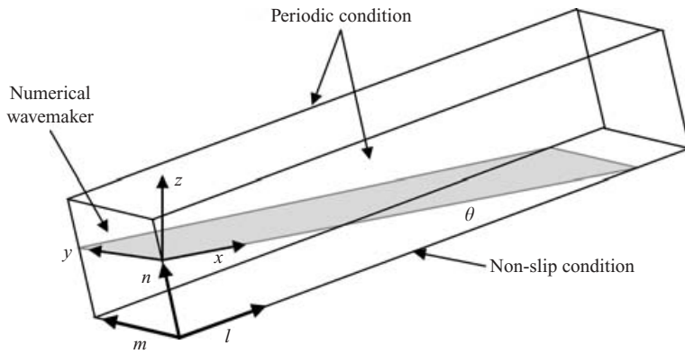
FIGURE 2. Computing domain and coordinate system.
