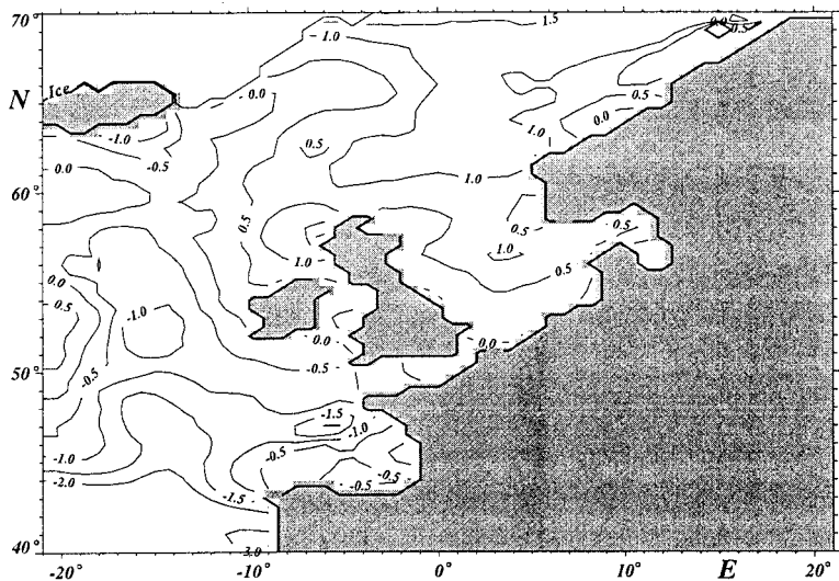
FIG. 11. Map of the 1955–94 trends in the intraannual 90% quantiles of significant wave height, as derived from the 40-yr hindcast executed with the WAM wave model. Units: cm yr -1 . (From Günther et al. 1998.)
