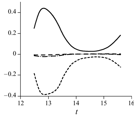
FIGURE 17. Temporal development of vertical integrated value of the terms of equation (14), R_\delta = 800 : —, production (term V); - - -, dissipation (term VI); - · - · -, turbulent convection (term III); - · - · -, diffusion (term IV).
