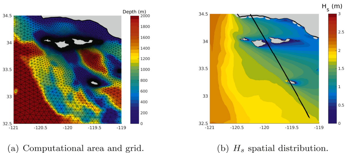
Fig. 4. SWAN computational area and the unstructured grid — colors represent water depth (a). In (b), one of the 31 coincident cases with peak wave direction \theta = 311^\circ for April 4 th 2015 at 05:00) showing the Channel Islands as an effective obstacle to the wave propagation — H_s down-wave is nearly zero in the vicinity of the archipelago. Jason-2 ground track depicted as the thick black line and the colors represent H_s .
