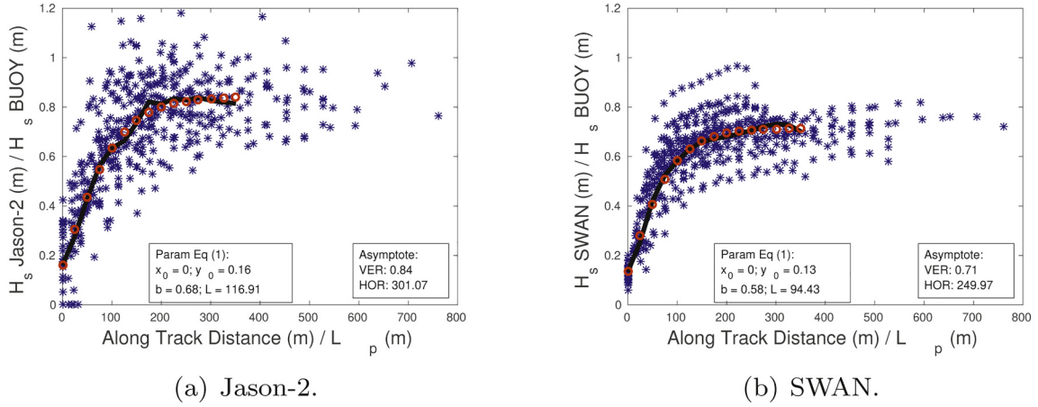
Fig. 6. The diffraction coefficient as a function of non-dimensional distance. The horizontal axis is the ratio between the along track distance in the lee of the archipelago and the peak wavelength L_p measured by the offshore buoy. The vertical axis is the ratio between the diffracted H_s measured by Jason-2 (a) or estimated by the numerical model (b) and the incident H_s measured by the same offshore buoy. The thick black line is the mean of the 31 coincident cases. The red circles depict the fit using Eq. (8). The values of the asymptote are also displayed (lower right corner panel) and the parameters of Eq. (8) (lower central panel). (For interpretation of the references to colour in this figure legend, the reader is referred to the web version of this article.)
