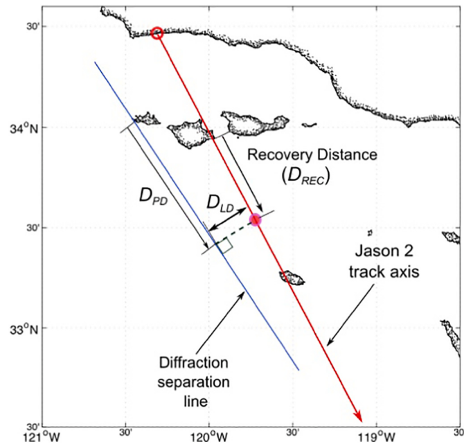
Fig. 9. The red line is the segment of Jason-2 ground track used in the study, whereas the blue line is a given peak wave direction at the offshore buoy — 324^\circ in the example depicted — tangent to the westernmost tip of the archipelago and designated as diffraction separation line. D_{REC} is the position of one of the computed recovery distances along the ground track — see Fig. 3(b). The orthogonal from D_{REC} up to the diffraction separation line is the distance of lateral diffraction D_{LD} — dashed line. Moreover, D_{PD} is the distance from the westernmost tip of the archipelago up to the projection of D_{REC} on the diffraction separation line. (For interpretation of the references to colour in this figure legend, the reader is referred to the web version of this article.)
