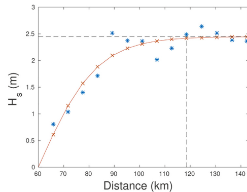
(b) Values of recovery distance and H_{s-lim} to reach the asymptote.
