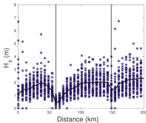
(a) H_s along the ground track shown in Figure 2 for the 41 selected cases.
