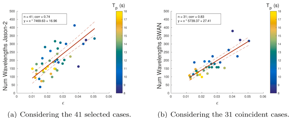
Fig. 8. Offshore buoy steepness \epsilon = \frac{H_s \pi}{L_p} against the number of wavelengths to reach the limit — ratio between the down-wave recovery distance (as shown in Fig. 3 (b)) and the offshore buoy peak wavelength L_p . In (a) Jason-2, in (b) SWAN. The red full line is the least-squares fit and the dashed lines indicate the 95% confidence intervals — equation shown on top of both plots. The colorbar is the offshore buoy peak period T_p . (For interpretation of the references to colour in this figure legend, the reader is referred to the web version of this article.)
