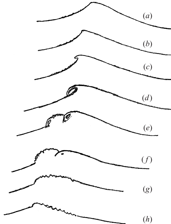
FIGURE 11. Schematics of breaking waves at the group peak, depicting various phases: steepening-crest phase (a); plunging-jet phase, (b), (c), (d); splashing-ploughing phase, (e), (f), (g); and decaying scar phase, (h).
