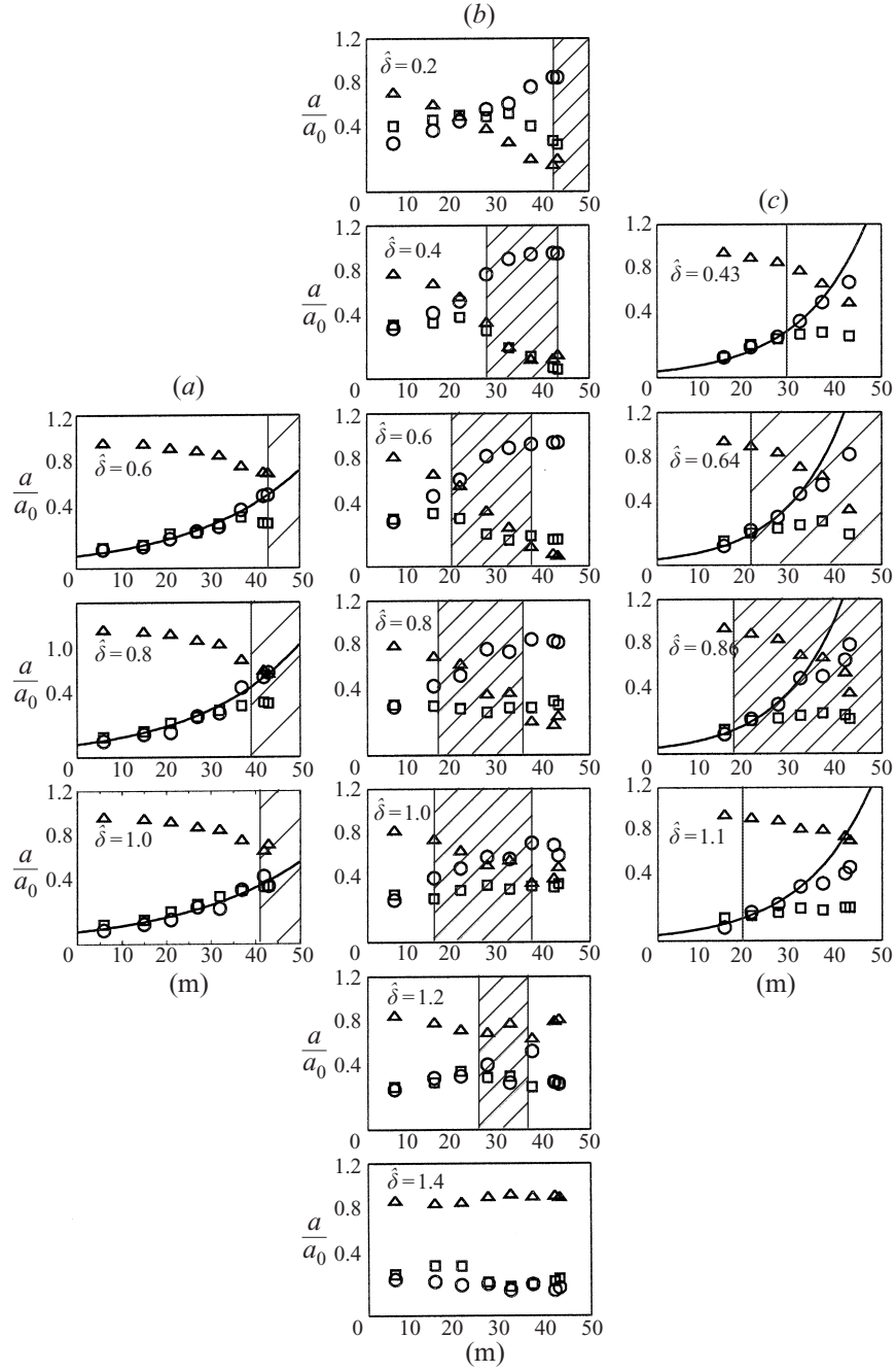
FIGURE 14. Evolution of wave modes for 2.3 m wave: (a) \epsilon = 0.165 , for \hat{\delta} = 0.6, 0.8 and 1.0 , b_{\pm}/a_0 = 0.1 ; (b) \epsilon = 0.165 , \hat{\delta} = 0.2, 0.4, 0.6, 0.8, 1.0, 1.2 , and 1.4 , b_{\pm}/a_0 = 0.3 ; (c) \epsilon = 0.28 , \hat{\delta} = 0.43, 0.64, 0.86 and 1.1 , b_{\pm}/a_0 = 0.05 . Shaded part indicates where the waves broke. Symbols are: \triangle , carrier; \circ , lower; \square , upper.
