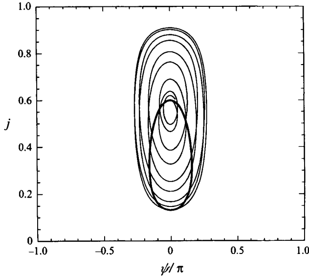
FIGURE 8. Numerically computed trajectory (j, \psi) (thin line) for \beta = 0.1 , r = 0.7 , j_* = 2 and \Delta = 0 . The system evolved from the initial condition (j, \psi) = (0.6, 0) until time t = 50 . The Poincaré map, sampling every long-wave period t = 2\pi n , is indicated by the thick curve.
