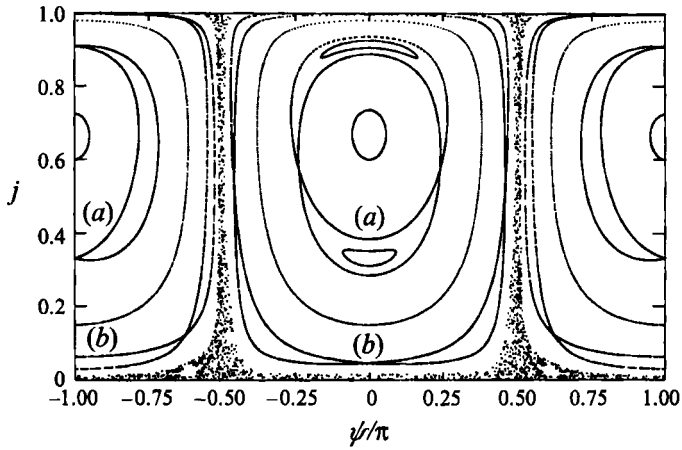
FIGURE 14. Poincaré map for r = 0.55 , j_* = 0 , \Delta = 0 , \beta = 0.01 . We see subharmonic \frac{1}{2} modulatory resonance (a) and subharmonic \frac{1}{3} modulatory resonance (b).
