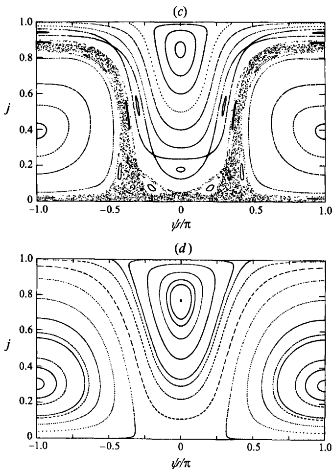
FIGURE 15. Poincaré map for r = 0.55 , j_* = 0 , \Delta = 0 : (c) \beta = 1.2 , (d) \beta = 2.0 .
