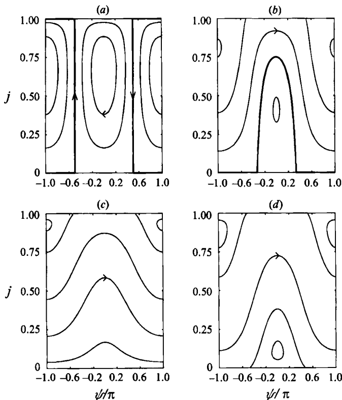
FIGURE 6. Phase portraits (j, \psi) for the autonomous system. (a) j_* = 0 , \Delta/r = 0 ; (b) j_* = 0 , \Delta/r = 0.5 ; (c) j_* = 0 , \Delta/r = 1.5 ; (d) j_* = 1 , \Delta/r = 1.5 . The homoclinic trajectory is drawn as a thick line in (a) and (b).
