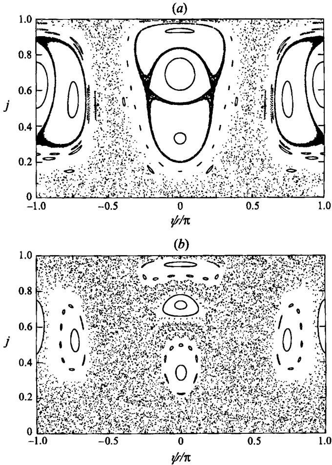
FIGURE 15. Poincaré map for r = 0.55 , j_* = 0 , \Delta = 0 : (a) \beta = 0.1 , (b) \beta = 0.2 .
