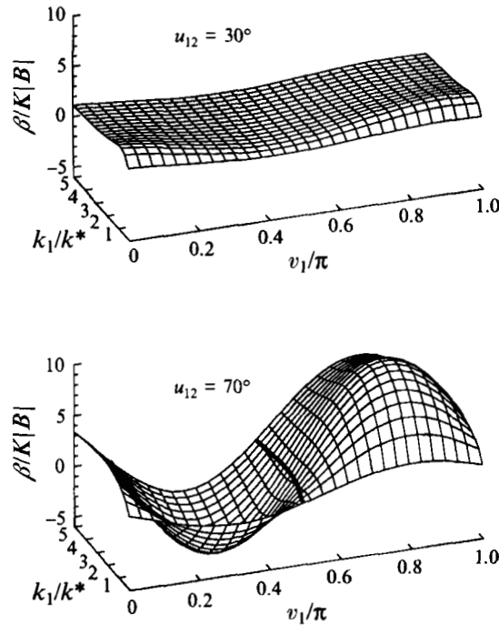
FIGURE 4. The effective long-wave/short-wave interaction coefficient \beta/K|B| as a function of the angle of incidence v_1/\pi and the wavenumber k_1/k^* in the range (0.1, 5.0) for two selected angles u_{12} = 30^\circ and u_{12} = 70^\circ . The zero crossings are indicated by thick contour lines.
