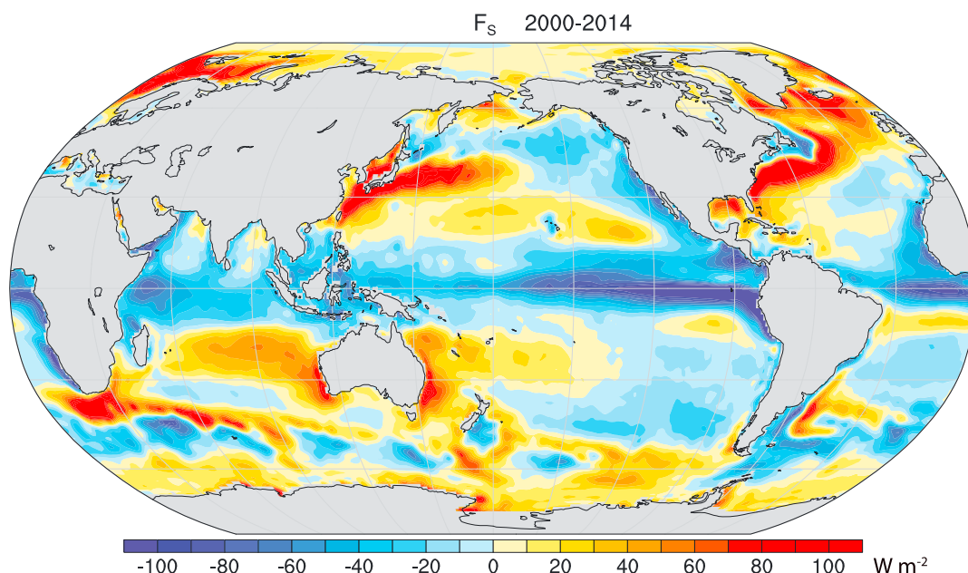
Figure 2. Surface heat flux: The net upward (from ocean to atmosphere) surface heat flux ( F_s ) for 2000–2014 in \text{W m}^{-2} .
