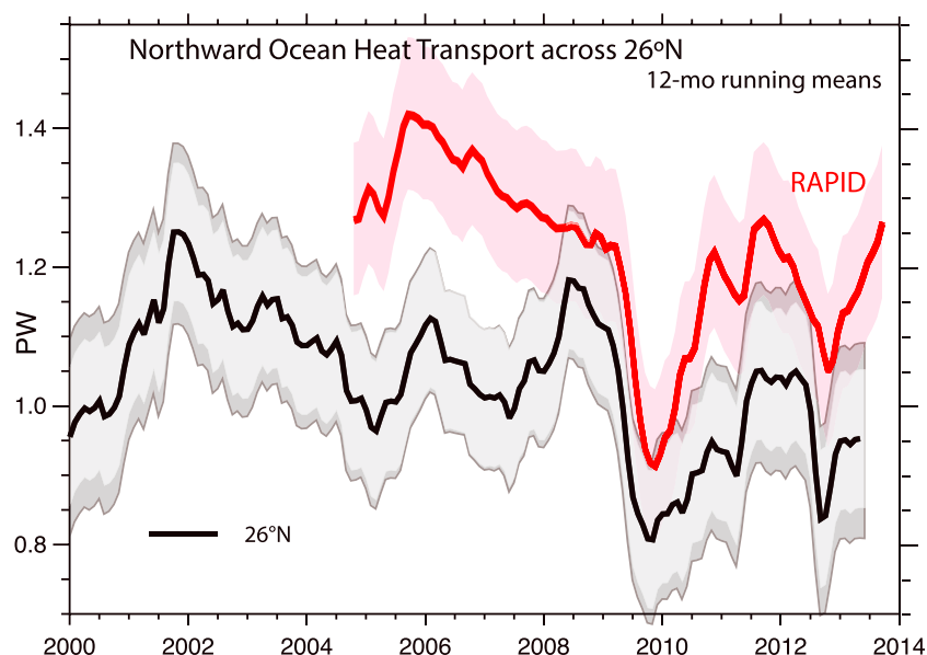
Figure 5. RAPID array heat transports: The 12 month running mean northward heat transports across 26^{\circ}\text{N} (black) from Figure 4 compared with results from the RAPID array (red) in PW. The error bars are \pm 1 standard deviation, for RAPID in pink, and for current results in gray, with a component (equivalent to a 0.42 \text{ W m}^{-2} trend) added to represent trend uncertainty (darker gray).
