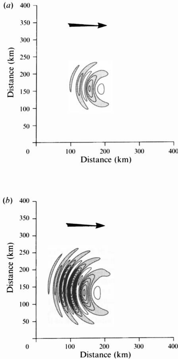
FIGURE 2. Kinetic energy (integrated over the mixed-layer depth and averaged one inertial period) for experiment D1, (a) at t = 10 inertial periods and (b) at t = 15 inertial periods. Contour interval is 0.02 \text{ m}^3 \text{ s}^{-2} . The shaded area shows energy levels higher than 0.08 \text{ m}^3 \text{ s}^{-2} . The wind direction is indicated by an arrow.
