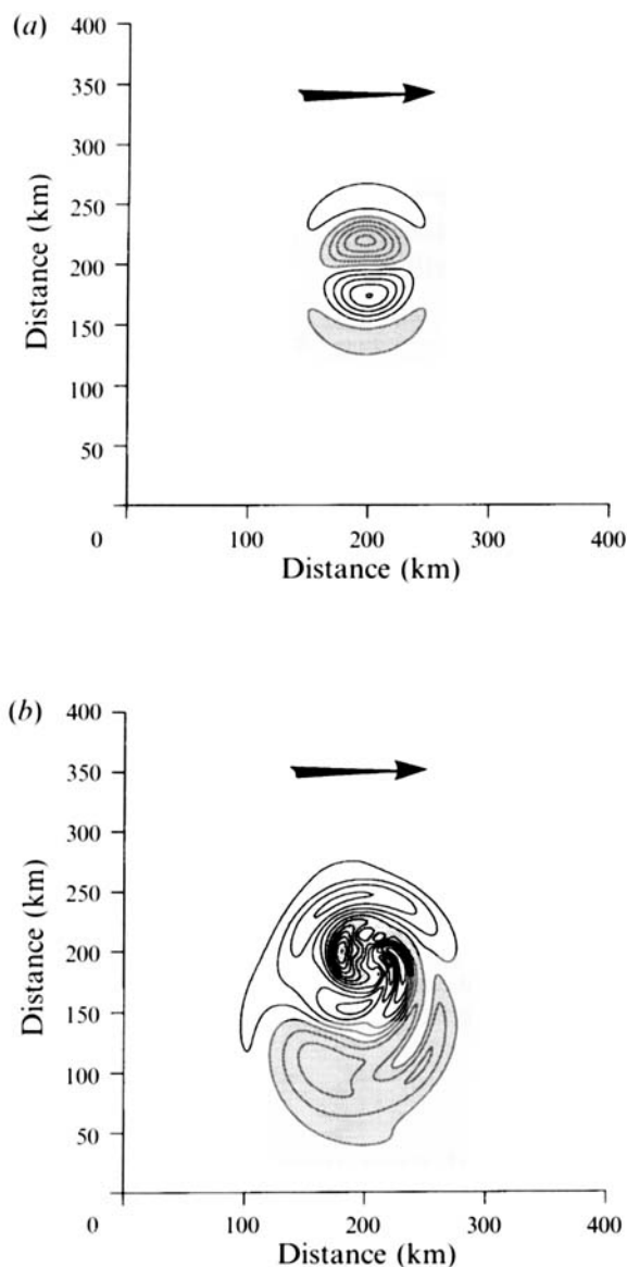
FIGURE 10. Mixed-layer depth perturbation h - h_0 for experiment C0, (a) at the end of the first inertial period. Contour interval is 0.3 m with minimum contour -1.35 m; (b) at the end of the 20th inertial period. Contour interval is 0.5 m with minimum contour -2.25 m. The shaded area indicates downwelling. The wind direction is indicated by an arrow.
