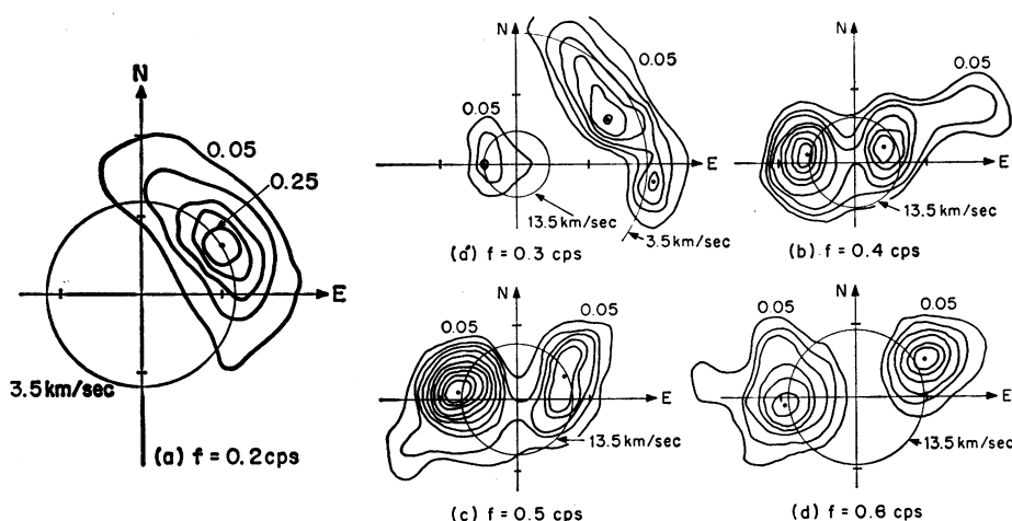
Fig. 1. Wave-number structure of microseisms on 2 December 1965. Coordinate axis is graduated in units of 0.05 cy/km.
