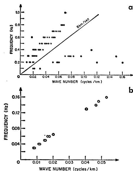
Fig. 3. (a) Cumulative frequency-wave number plot of microseism power peaks arriving from the west. Note the separation of surface waves and body waves on two sides of 8-km/sec line. (b) Frequency-wave number dispersion curve for the long-period vertical motion of microseisms; it corresponds to fundamental-mode Rayleigh-wave dispersion.
