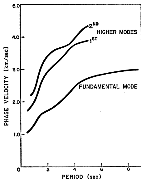
Fig. 2. Theoretical Rayleigh-wave dispersion curves for an average structure of LASA.
