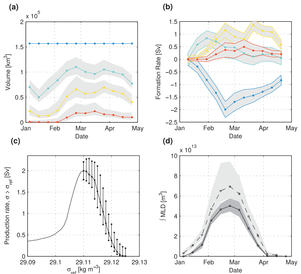
Figure 9. (a) Temporal evolution of the volume for waters presenting greater densities than 28.3 kg/m 3 (blue) corresponding to the minimum density observed in the deep convection area shown in Figure 8, 29.11 kg/m 3 (green), 29.115 kg/m 3 (yellow), and 29.12 kg/m 3 (red). Error bars in gray result from the optimal interpolation error. (b) Temporal evolution of the volume of water between consecutive isopycnals calculated by comparison to the situation on 5 January and reduced to Sv (volume averaged over 1 year) for waters presenting densities lower than 29.11 kg/m 3 (blue), between 29.11 kg/m 3 and 29.15 kg/m 3 (green), between 29.115 kg/m 3 and 29.12 kg/m 3 (yellow), and greater than 29.12 kg/m 3 (red). Error bars result from those of Figure 9a. (c) Volume of water denser than a given isopycnal produced between the 5 January and 24 February. Error bars are computed from the volume error of each density class of the optimal interpolation. For clarity, they are only plotted for waters undergoing a net volume increase during considered period. (d) Convective volume defined as the volume-integrated mixed layer. The continuous line represents this quantity for MLD greater than 1,000 m and the dashed line for MLD greater than 500 m. Error bars in gray result from the optimal interpolation error.
