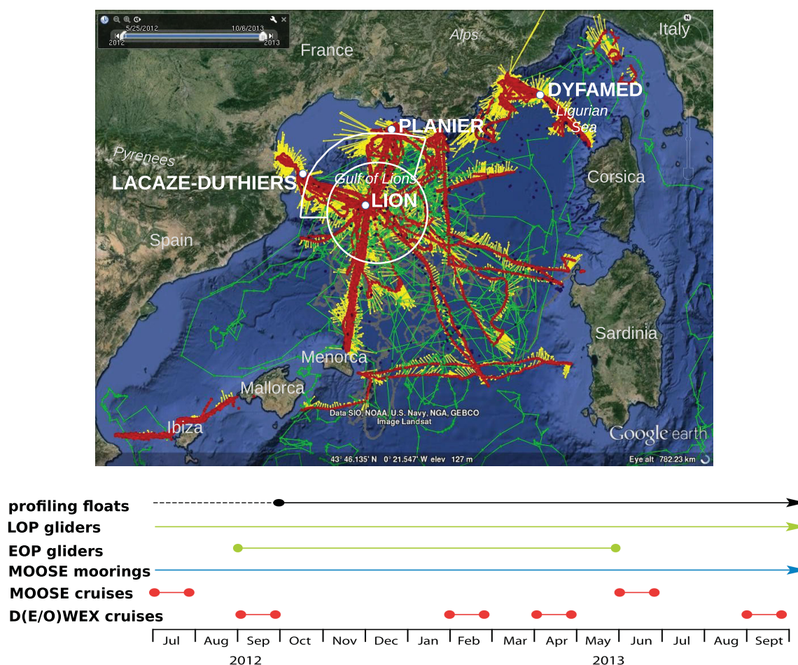
Figure 1. All observations carried out between 1 July 2012 and 1 October 2013. Gliders surface positions (red dots) and measured depth-average currents (yellow arrows). Profiling floats surface positions and trajectories (green). CTD casts from research cruises (blue). Surface drifters trajectories (grey). Positions of the LION, LACAZE-DUTHIERS, PLANIER, and DYFAMED moorings (white dots). The two selection areas “Boundary Current” and “Mixed Patch” used in Figure 4 are displayed in white.
