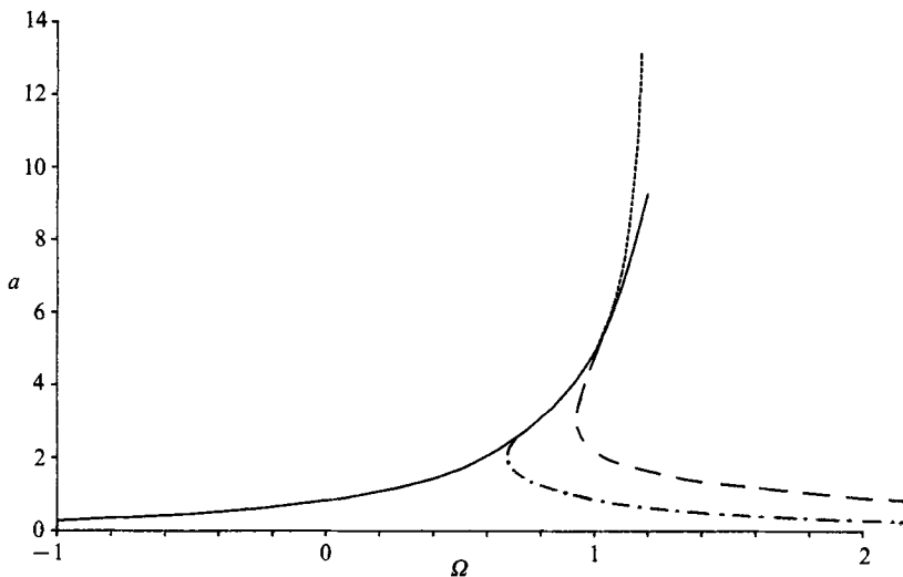
FIGURE 11. Curves in the vorticity, wave-height plane: —, Extreme solitary waves; ----, Highest solitary waves; —·—, Solitary waves with zero pressure gradients at their crests; ·····, Line separating solitary waves with eddies (above) from those without.
