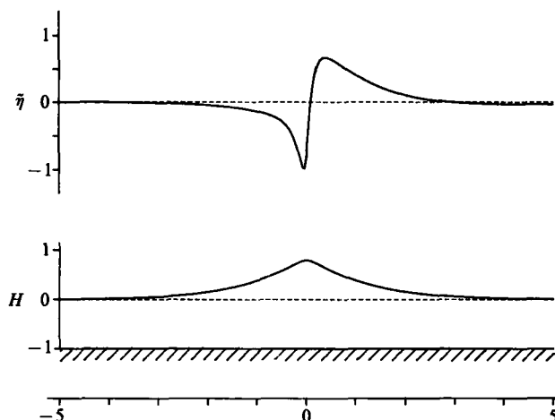
FIGURE 1. Growing normal-mode perturbation \tilde{\eta}(x) for a solitary wave (shown beneath to natural scale) propagating from right to left. The decaying mode is given by -\tilde{\eta}(-x) .
