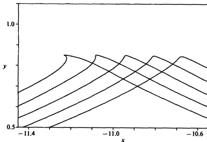
FIGURE 5. Overturning of the breaking wave crest ( \epsilon = -0.01 ). Profiles are shown at times t = 8.5, 8.6, 8.7, 8.8 and 8.9 .
