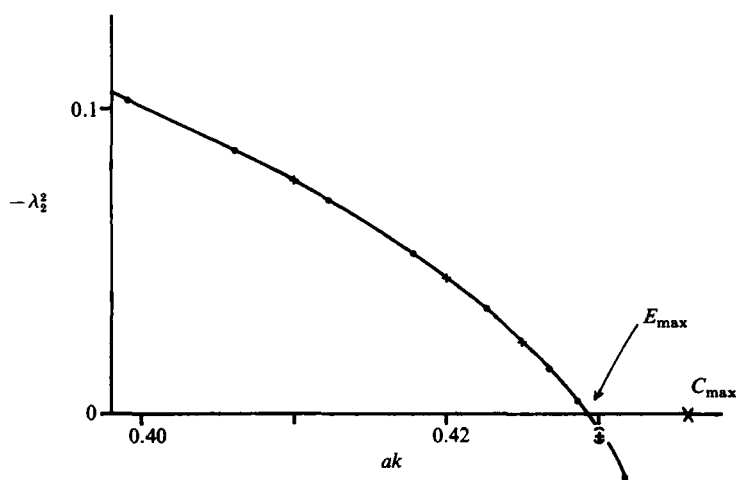
FIGURE 1. Graph of the squared eigenvalue -\lambda^2 versus ak . \bullet\bullet\bullet , our previous results (1983); + , present results. The bracket attached at ak = 0.43 roughly indicates the numerical inaccuracy involved.
