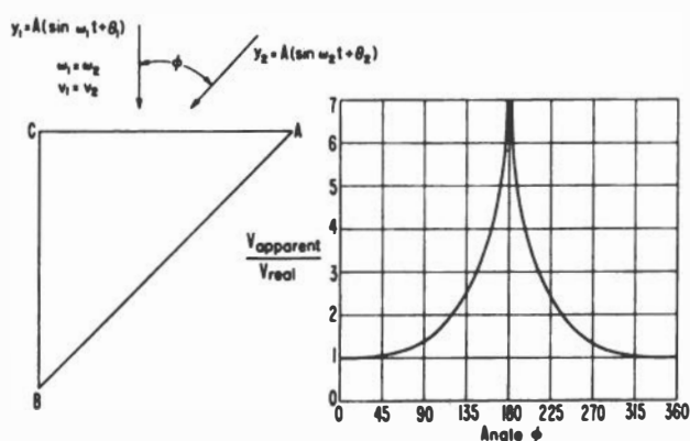
Figure 2. Ratio of apparent velocity to real velocity as a function of angle between direction of propagation of two similar wave trains.
