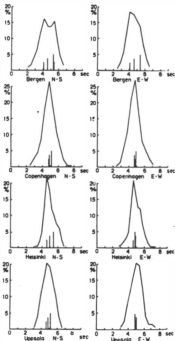
Figure 3. Period spectra on October 28, 1947, at 07 h M.E.T.
