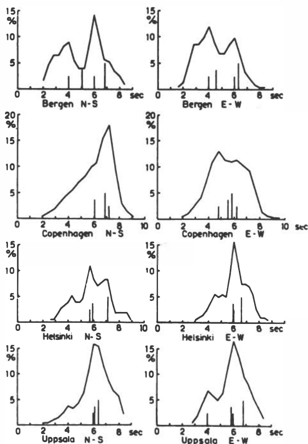
Figure 5. Period spectra on March 23, 1949, at 07 M.E.T.
