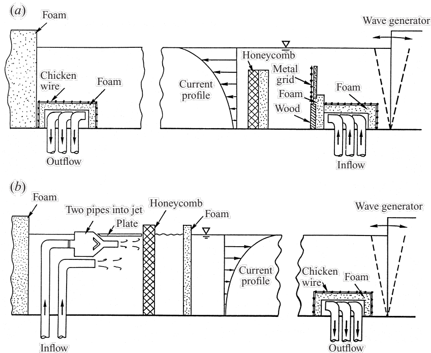
FIGURE 2. Inlet conditions: (a) generation of waves on a 'favourable' shear current; (b) generation of waves on an 'adverse' shear current.
