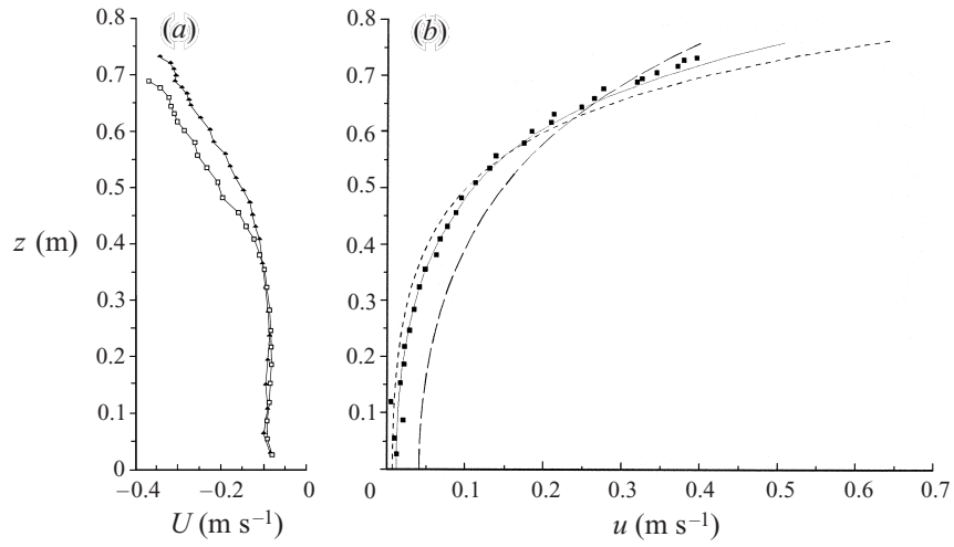
FIGURE 9. Interactions with a strongly sheared 'adverse' current, case 10. (a) Current profile: \square , initial current; \blacktriangle , current measured in presence of waves. (b) Wave kinematics: \blacksquare , horizontal velocity measured beneath wave crest; ---, waves-only solution, U = 0 ; ·····, Doppler-shifted solution, U = U_s ; —, multi-layered numerical model, U = U(z) .
