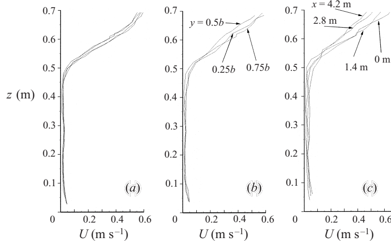
FIGURE 4. Measurements of a 'favourable' current profile, U . (a) Time variation, U(t) ; (b) cross-tank variation, U(y) , where y is measured from the sidewall and b is the flume width; (c) downstream variation, U(x) .
