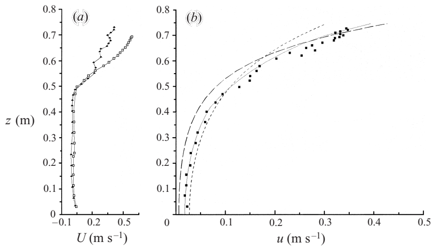
FIGURE 6. Interactions with a strongly sheared 'favourable' current, case 5. (a) Current profile: \square , initial current; \blacktriangle , current measured in presence of waves. (b) Wave kinematics: \blacksquare , horizontal velocity measured beneath wave crest; --- , waves-only solution, U = 0 ; \cdots , Doppler-shifted solution, U = U_s ; — , multi-layered numerical model, U = U(z) .
