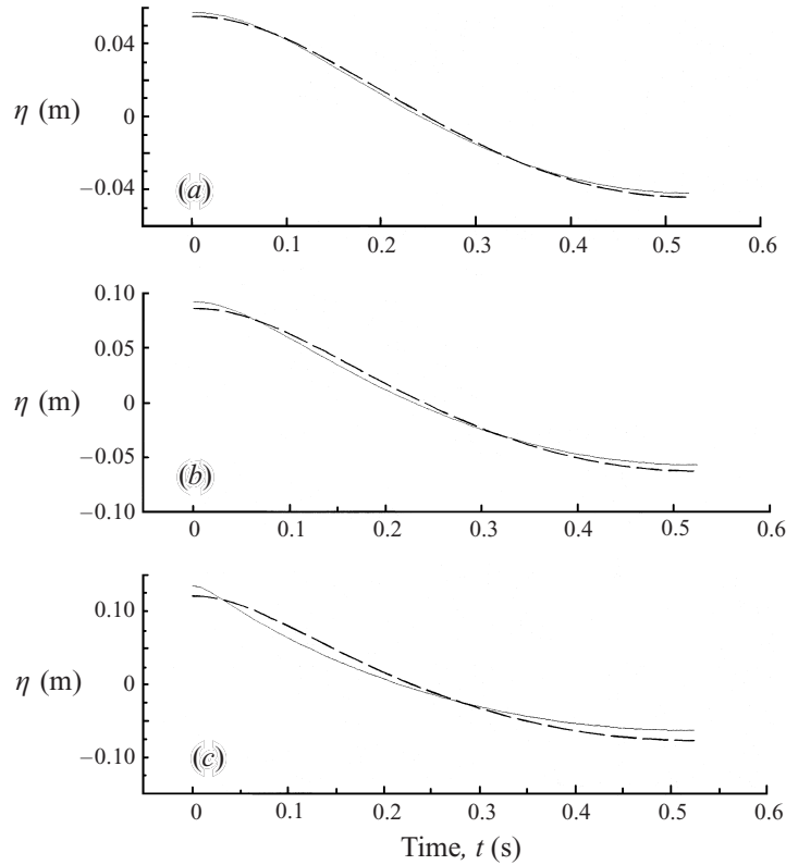
FIGURE 13. Surface elevations, \eta(t) , for waves ( T = 1.05 s) on current case 7. (a) H = 0.10 m; (b) H = 0.15 m; (c) H = 0.20 m. — — —, Waves-only solution, U = 0 ; —, multi-layered numerical model, U = U(z) .
