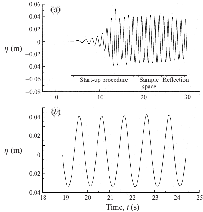
FIGURE 3. Water surface elevations, \eta(t) , recorded on a strongly sheared 'adverse' current: (a) long-term evolution ( 0 \leq t \leq 30 s) showing initial start-up, sample space and the arrival of unwanted reflections; (b) close-up of sample space ( 19 \text{ s} \leq t \leq 24 \text{ s} ).
