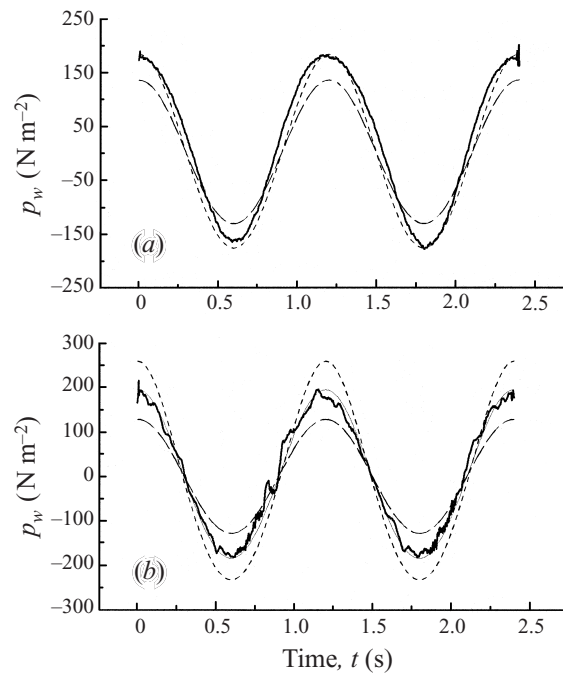
FIGURE 14. Wave-induced pressure fluctuations measured at the bed, p_w . (a) Waves on a uniform current, current case 3; (b) waves on a 'favourable' shear current, current case 5. —, Experimental data; — —, waves-only solution, U = 0 ; ·····, Doppler-shifted solution, U = U_s ; ———, multi-layered numerical model, U = U(z) .
