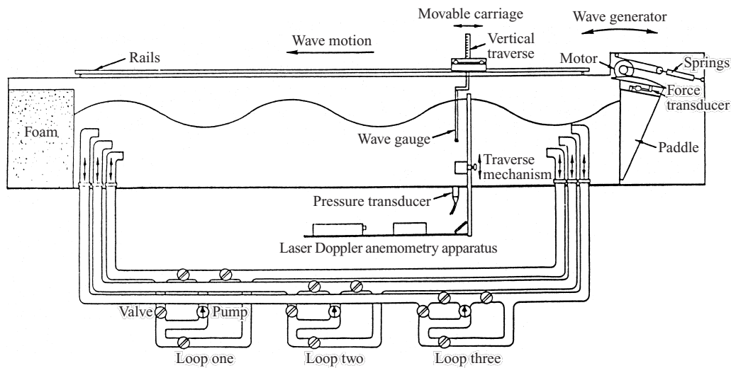
FIGURE 1. Side view of the experimental apparatus.
