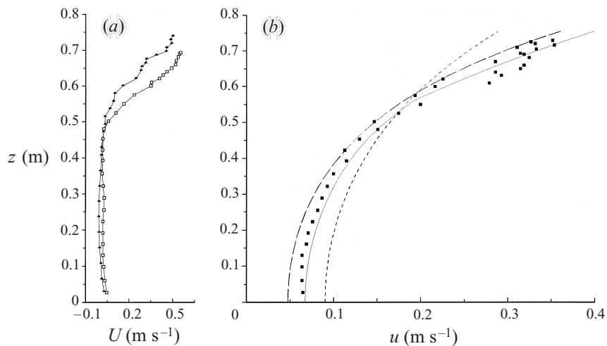
FIGURE 8. As figure 6 but for case 7.
