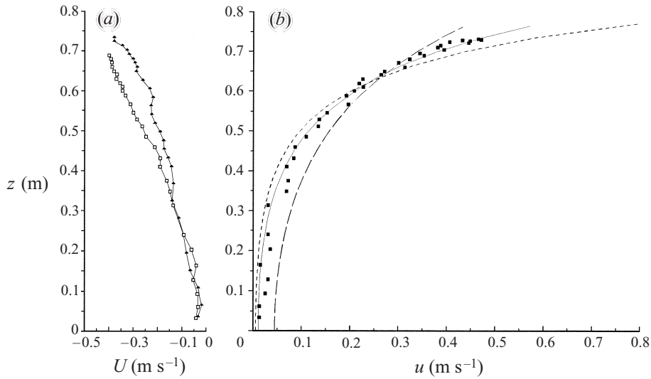
FIGURE 10. As figure 9 but for case 11.
