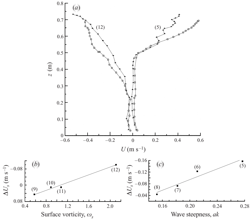
FIGURE 12. Changes in the current profile. (a) U(z) , cases 5 and 12: \square , initial current; \blacktriangle , current measured in presence of waves. (b) Current change, \Delta U_s , vs. surface vorticity, \omega_s . (c) Current change, \Delta U_s , vs. wave steepness, ak . Number in brackets refers to case.
