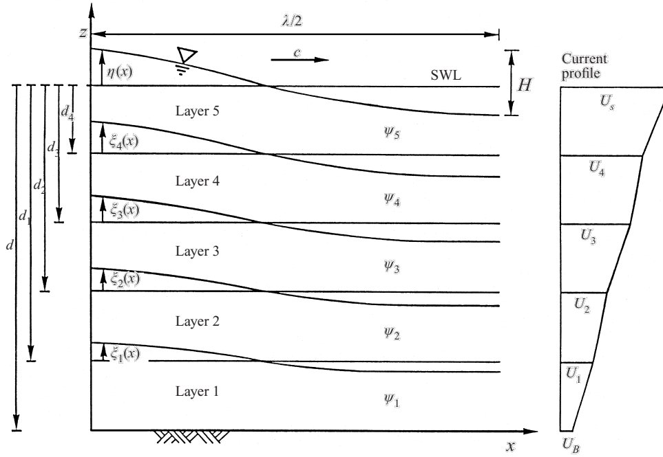
FIGURE 17. Coordinate arrangement and solution domain. (Note: Within this solution z is measured from the still water level upwards.)
