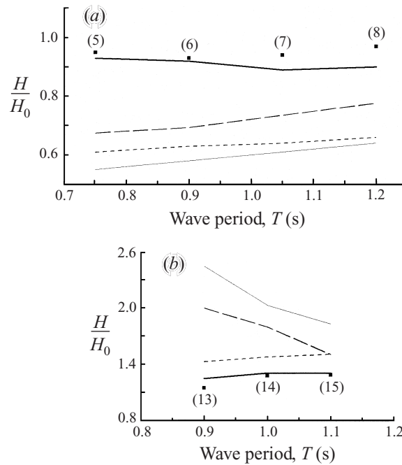
FIGURE 16. Wave height changes. (a) Waves on a 'favourable' shear current, cases 5–8; (b) waves on an 'adverse' shear current, cases 13–15. ■, Experimental data; —, O(\varepsilon) Doppler-shifted solution, U = U_s ; - - - - -, O(\varepsilon^5) Doppler-shifted solution, U = U_s , Thomas (1990); - · - · -, O(\varepsilon^2) constant vorticity solution, U = U_s - \Omega(z-d) , Jonsson et al. (1978); —, multi-layered numerical model, U = U(z) .
