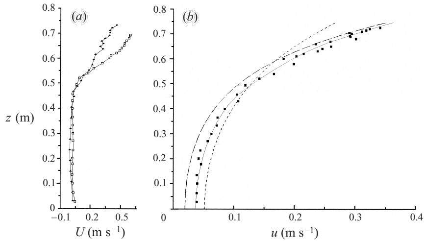
FIGURE 7. As figure 6 but for case 6.
