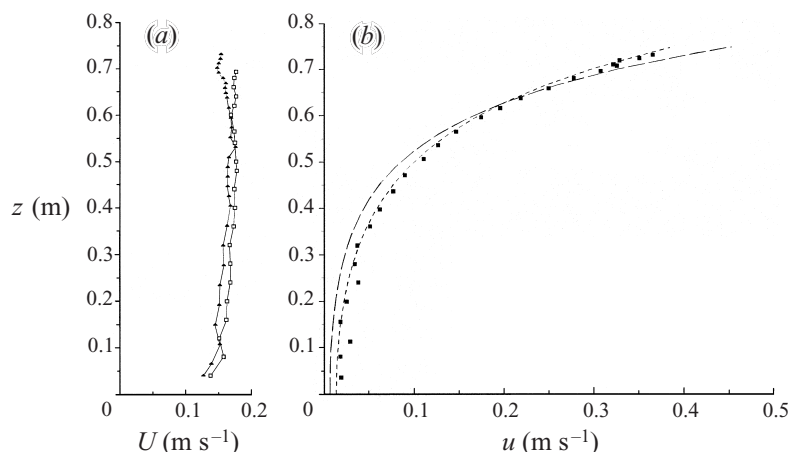
FIGURE 5. Interactions with a 'favourable' uniform current, case 3. (a) Current profile: \square , initial current; \blacktriangle , current measured in presence of waves. (b) Wave kinematics: \blacksquare , horizontal velocity measured beneath wave crest; ---, waves-only solution, U = 0 ; - · - · -, Doppler-shifted solution, U = U_s .
