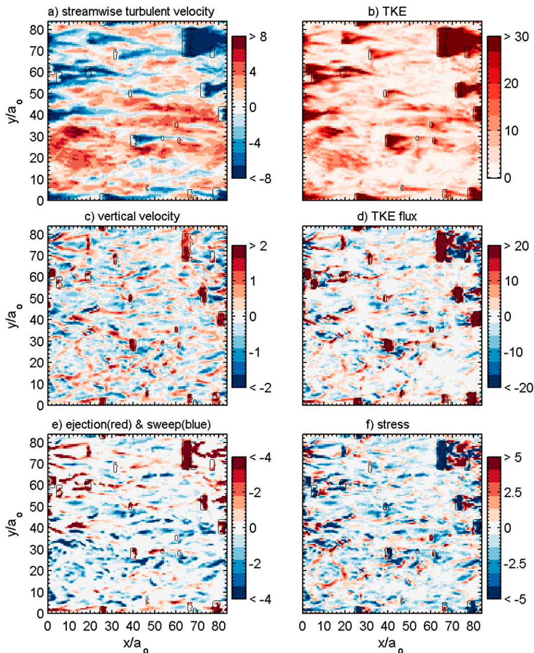
FIG. 4. Example snapshots of the instantaneous turbulence fields on a horizontal plane at z/a_o = 5/9 (where a_o = 1.40 m) from a simulation having U_{10} = 59 \text{ m s}^{-1} and (f_b, C_D^{\text{UN}}, \text{ and } \lambda_o) = (6, 0.0006, \text{ and } 29.22 \text{ m}) : (a) \overline{u'}/U_* , (b) normalized TKE, (c) \overline{w'}/U_* , (d) f_T/U_*^3 , (e) ejection ( \overline{u'w'}/U_*^2 , where \overline{u'} < 0 and \overline{w'} > 0 ) and sweep ( \overline{u'w'}/U_*^2 , where \overline{u'} > 0 and \overline{w'} < 0 ), and (f) (\overline{u'w'} + R_{13})/U_*^2 . The black solid contours indicate the location of the resolved breakers (the breaker forces).
