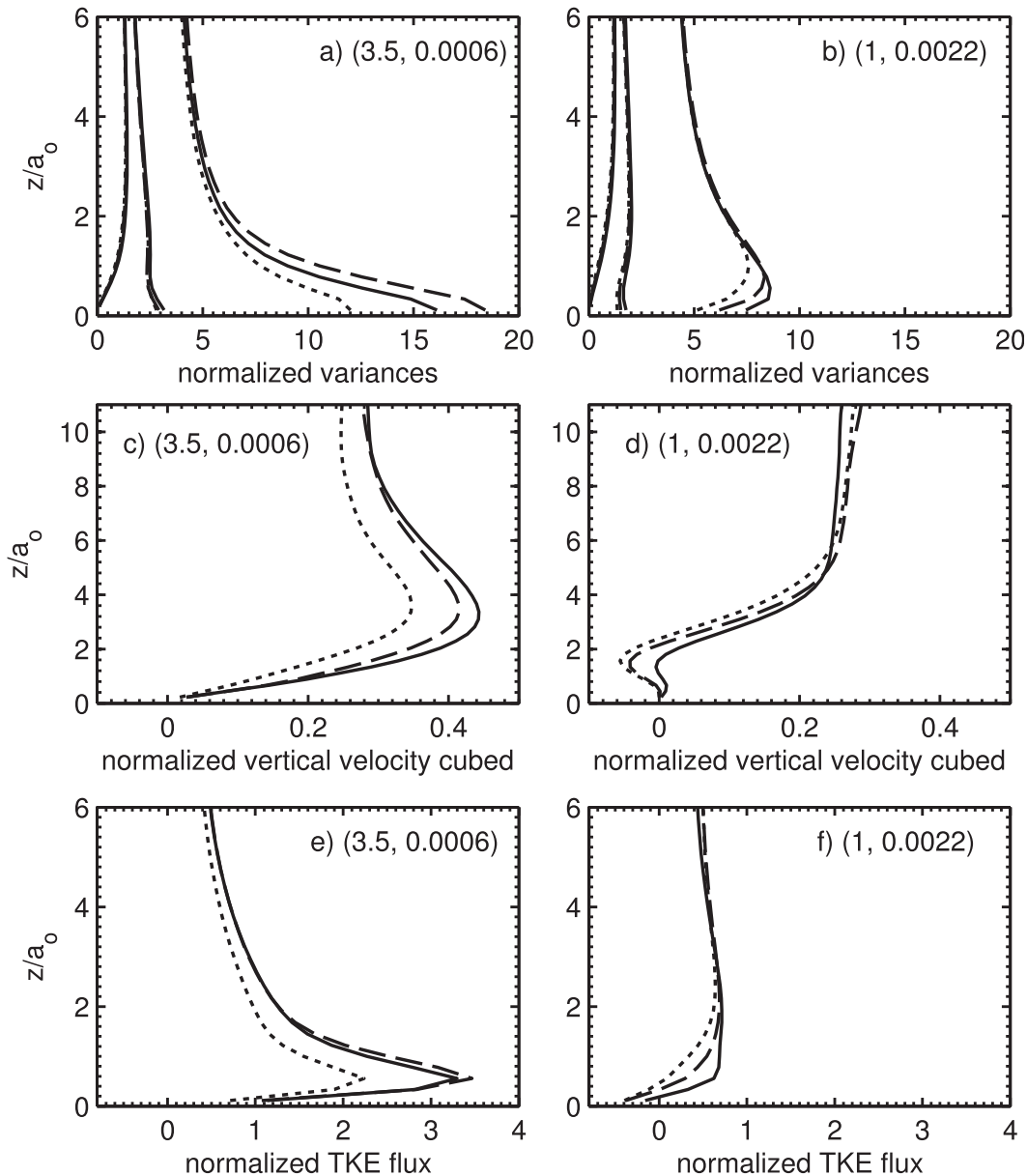
FIG. 5. (a),(b) \langle \overline{u'u'} \rangle / U_*^2 (largest), \langle \overline{v'v'} \rangle / U_*^2 (intermediate), and \langle \overline{w'w'} \rangle / U_*^2 (smallest). (c),(d) \langle \overline{(w')^3} \rangle / U_*^3 . (e),(f) \langle f_T \rangle / U_*^3 . Parameters (f_b, C_D^{\text{RN}}) = (3.5, 0.0006) for (a),(c), and (e) and (1, 0.0022) for (b),(d), and (f). The dotted lines are at U_{10} = 17 \text{ m s}^{-1} and \lambda_o = 29.22 \text{ m} ( a_o = 1.40 \text{ m} ). The dashed lines are at U_{10} = 59 \text{ m s}^{-1} and \lambda_o = 29.22 \text{ m} ( a_o = 1.40 \text{ m} ). The solid lines are at U_{10} = 59 \text{ m s}^{-1} and \lambda_o = 256.46 \text{ m} ( a_o = 12.24 \text{ m} ).
