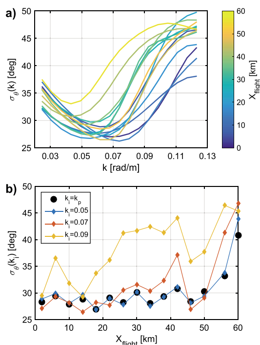
Figure 5. Directional spreading of wavenumber spectra. (a) Spectral spreading, \sigma_\theta(k) , as a function of wavenumber (equation (10)). Each curve corresponds to a 4 km flight segment; the color indicates X_{\text{flight}} . (b) Spectral spreading at chosen wavenumbers, k_i , as functions of X_{\text{flight}} . The black circles are the spreading at k_i = k_p , the blue diamonds are at k_i = 0.05 rad/m, the red diamonds are at k_i = 0.07 rad/m, and the yellow diamonds are at k_i = 0.09 rad/m.
