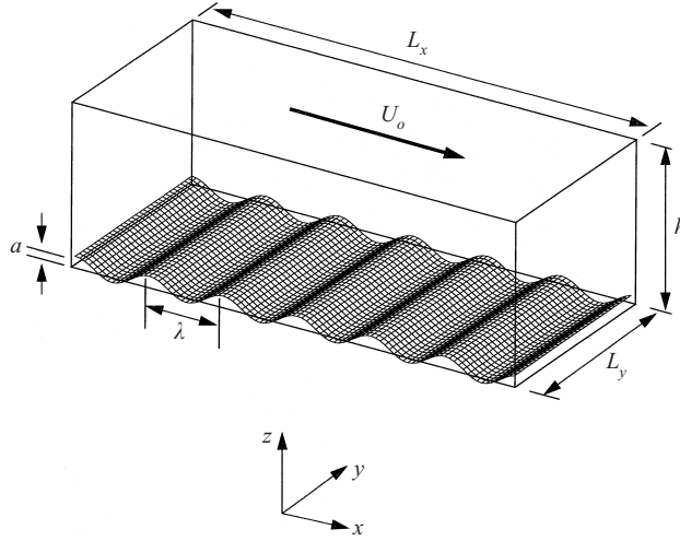
FIGURE 1. Sketch of three-dimensional Couette flow driven by velocity U_o over a moving wavy boundary of wavelength \lambda (or wavenumber k = 2\pi/\lambda ), phase speed c , and amplitude a in a domain of size (L_x, L_y, h) = (6, 5, 1)\lambda . For clarity, the surface grid is shown with less resolution than actually used in the computations.
