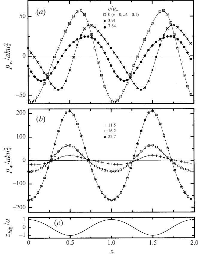
FIGURE 23. (a, b) Normalized wave-correlated surface pressure p_w/aku_*^2 for flow over surface waves with ak = 0.1 and varying c/u_* = 0, 3.9, 7.8, 11.5, 16.2, 22.7 . The normalized wave shape z_{bdy}/a is shown in (c).
