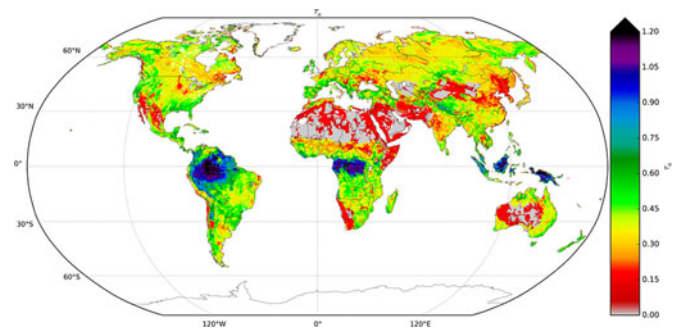
Fig. 1. Global map of average ASCAT vegetation optical depth over 2007–2011, cf. [16].
