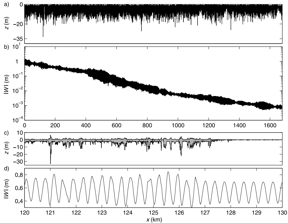
Figure 2. (a) The draft profile from the 1994 [NSIDC, 2006] data with all gaps filled; (b) the magnitude of the vertical displacement |W| of a 22 s ocean wave train as it progresses through ice terrain for the entire 1670 km transect; (c) a 10 km example of the thickness profile used in the model, showing ridge sails and keels; and (d) 10 km detail of the displacement magnitude |W| . Each are plotted against the horizontal coordinate x .
