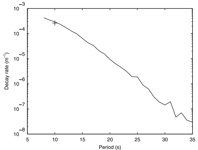
Figure 4. The rate of decay (attenuation coefficient, \alpha ) as a function of T . The cross plotted just below the curve at T = 10 \text{ s} shows \alpha when viscosity \gamma = 0 , i.e., when the decay is all due to scattering.
