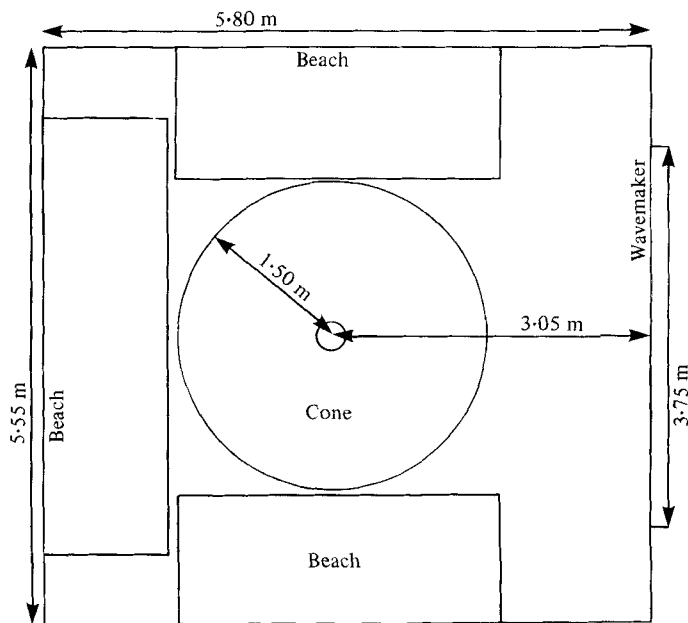
FIGURE 1. Plan of Provis's (1975) experiment.
