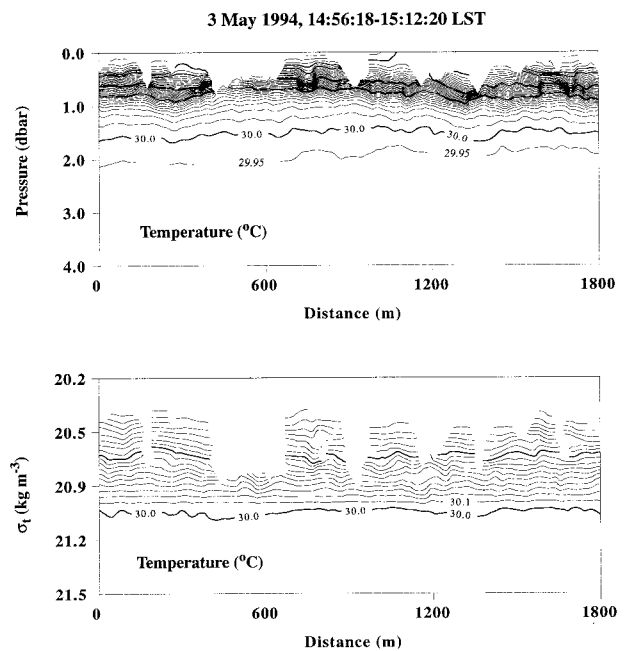
FIG. 14. Contour plots of T vs P and of T vs \sigma_t calculated during strong diurnal warming of the upper 1-m layer of the ocean (wind speed 2.2\text{--}2.4 \text{ m s}^{-1} , ship speed 2.0 \text{ m s}^{-1} ).
