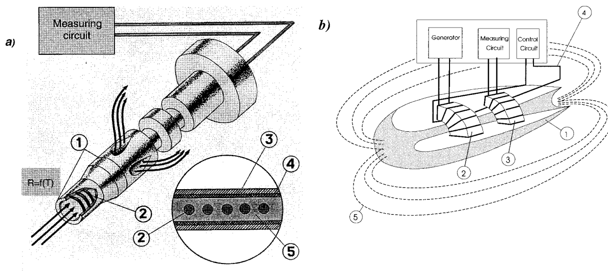
FIG. 3. (a) Construction of the primary temperature sensor: 1) the locations of laser welds, 2) the copper microwire of 20- \mu m diameter, 3) titanium body with 100- \mu m -thick walls, 4) isolation cover by nitride of silicon, and 5) compound filling. The balloon shows a cross section of the sensitive element wall in more detail. (b) Theoretical field of the inductive conductivity cell: 1) the epoxy body of the cell, 2) voltage transformer, 3) current transformer, 4) control winding, and 5) the “conducting loop.”
