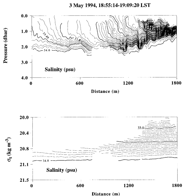
FIG. 15. Contour plots of S vs P and of S vs \sigma_t calculated during intersection of a surface freshwater lens (wind speed 2.7\text{--}4.6 \text{ m s}^{-1} , ship speed 2.4 \text{ m s}^{-1} ).
