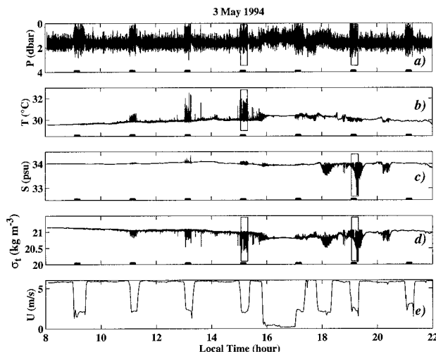
FIG. 12. Example of record made by bow sensors in the western Pacific warm pool (along 147^\circ\text{W} ) for a strong diurnal warming event. (a) Pressure, (b) temperature, (c) salinity, (d) density, and (e) ship speed. Segments marked by the boxes are used to plot the contour plots in Fig. 14 and 15. LST is for 147^\circ\text{W} longitude.
