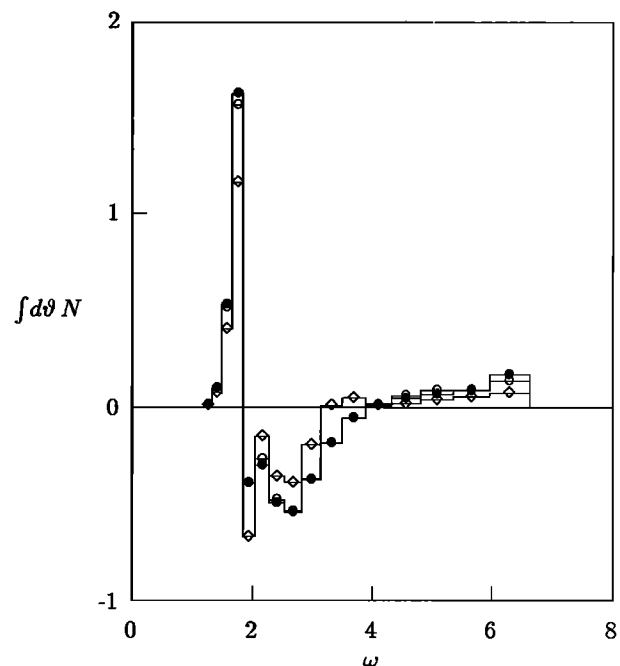
Fig. 10. Effect of k -scaled size-ordered truncation on integrated action transfer. Units and input spectrum as in Figure 1. Case-55 truncation. Number of coefficients is 50,000 (diamond), 100,000 (circle), and (no truncation) 170,662 (bullet).
