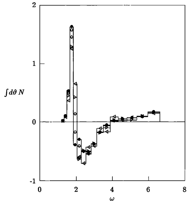
Fig. 2. Integrated action transfer for various resolutions of the integration grid. Units and input spectrum as in Figure 1. NWNH is 384. NTHH is 30 (left-pointing triangle), 50 (right-pointing triangle), 90 (diamond), 170 (circle), and 330 (bullet).
