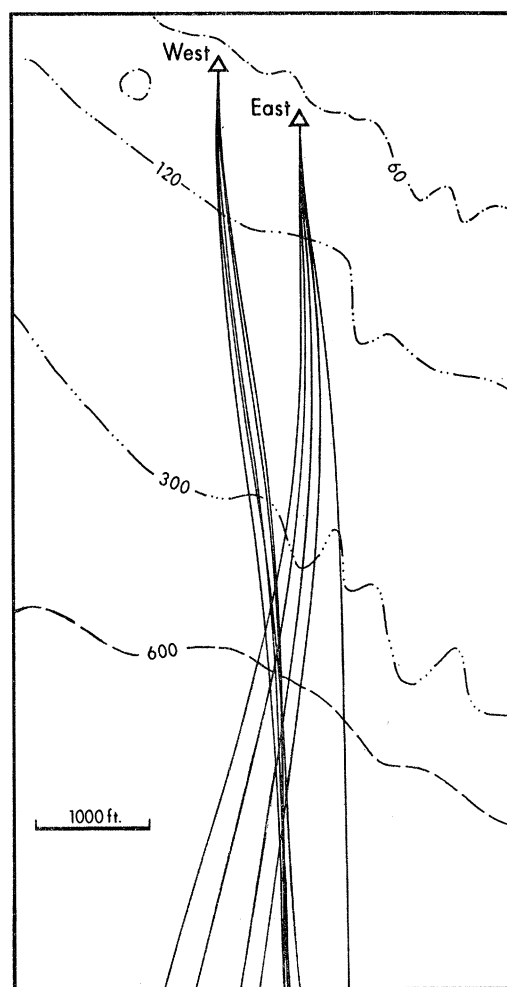
FIGURE 12. The refraction of waves of frequency 50 mc/s in the region shown in figure 5. Rays are drawn for directions 177^\circ , 178^\circ , ..., 181^\circ at the two instrument sites. Some selected depth contours (in feet) are drawn.
