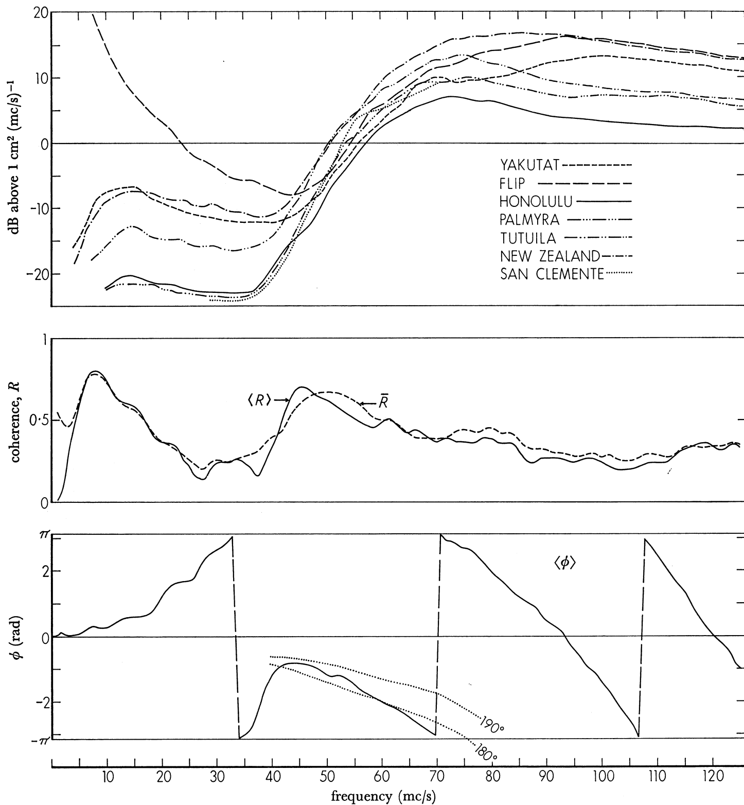
FIGURE 32. The mean wave field for September 1963, and for San Clemente Island during the month of August 1959. \langle R \rangle and \langle \phi \rangle are the coherence and phase of the mean wave field; \bar{R} is the mean coherence (see text). The dotted curves show \phi(f) for various offshore directions.
