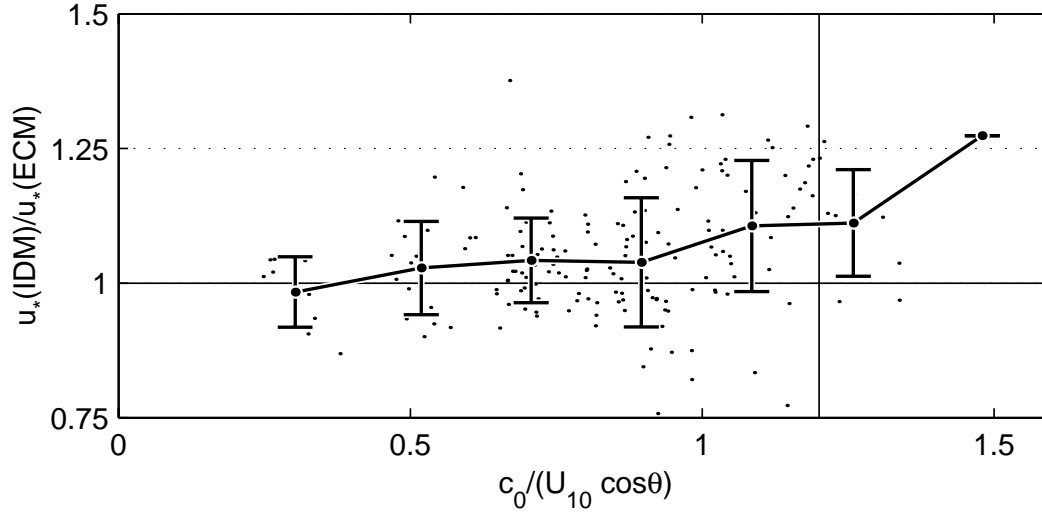
Figure 9: u_* from the inertial dissipation method divided by u_* from the eddy-correlation method as a function of wave age. The dots ( \bullet ) are all the measurements (from Paper III).
