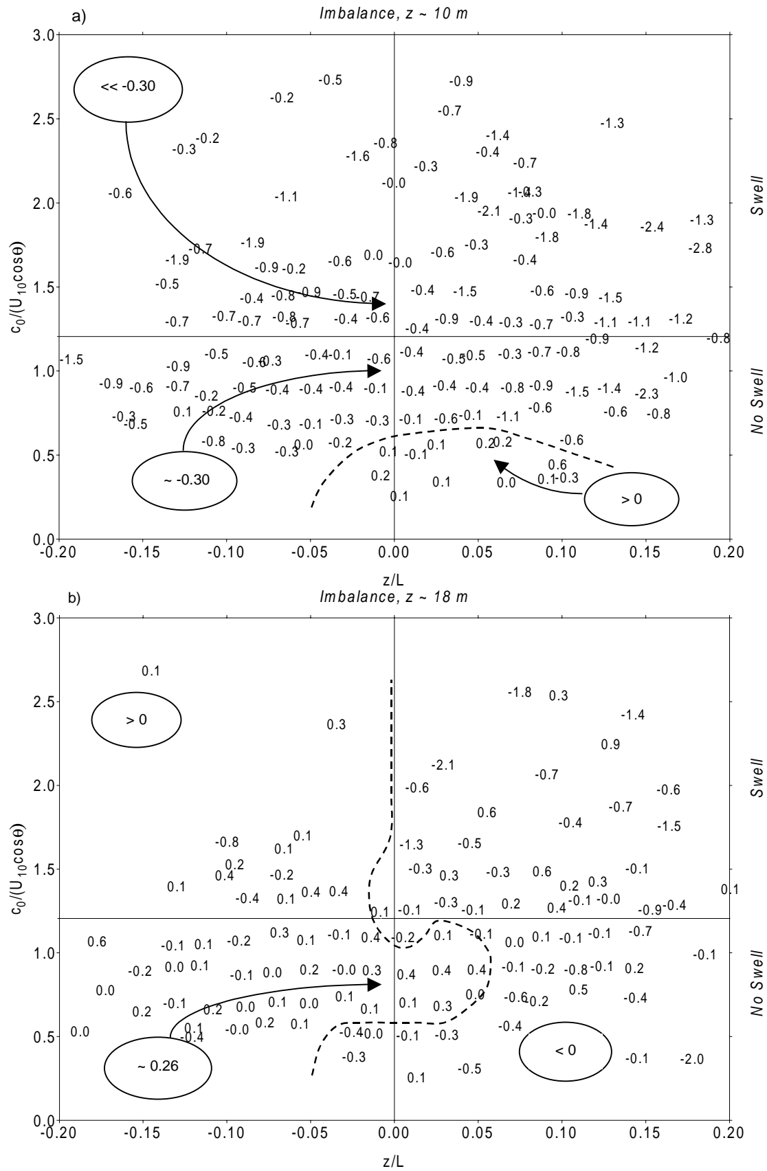
Figure 6: Imbalance as a function of z/L and c_0/(U_{10}\cos\theta) . a) Level 1, b) Level 2 and c) Level 3. Dashed line (--) shows imbalance \sim 0 .
