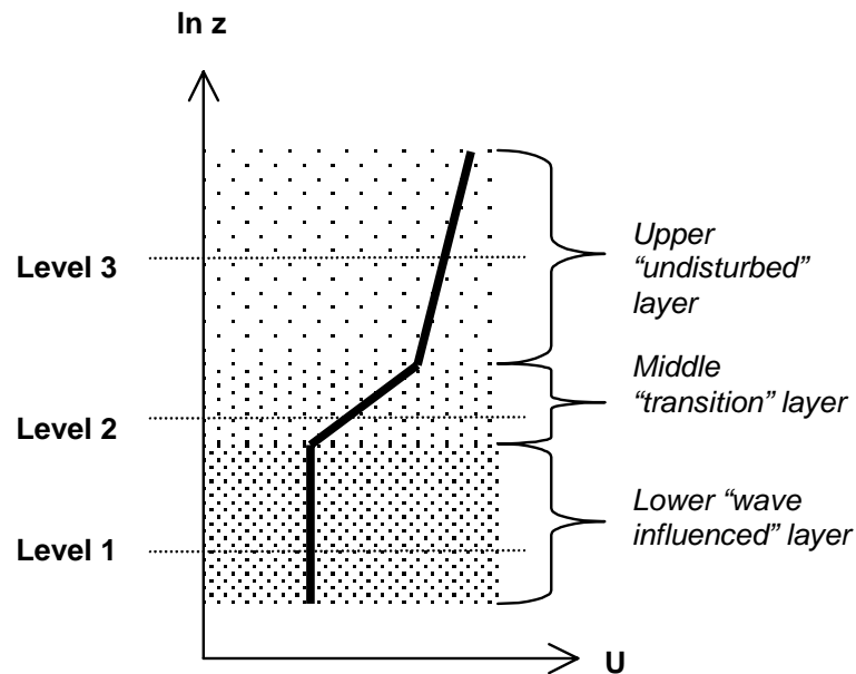
Figure 2: Typical appearance of a wind profile over the sea.
