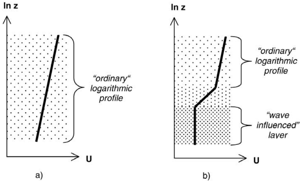
Figure 9. Two typical examples of wind profiles (schematically) during neutral conditions: (a) Growing sea with an 'ordinary' logarithmic profile, (b) swell with a wave influenced layer.
