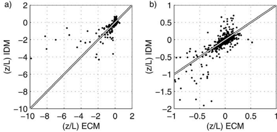
Figure 2. The stability parameter z/L from the eddy-correlation method (ECM) and the inertial dissipation method (IDM). Filled circles (●) are the measurements: (a) All data, (b) a close up of data between -1 < z/L < 1 .
