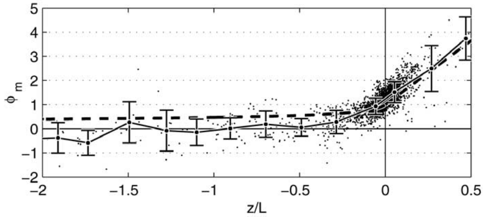
Figure 8. Normalised wind gradient \phi_m as a function of stability. Symbols as in Figure 5, dashed line (--) is the curve of Högström (1996). After Sjöblom and Smedman (2002).
