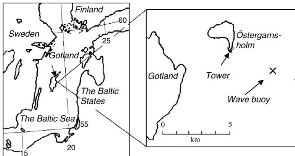
Figure 1. Map of the Baltic Sea, with a close up on Östergarnsholm. The location of the wave buoy is also indicated.
