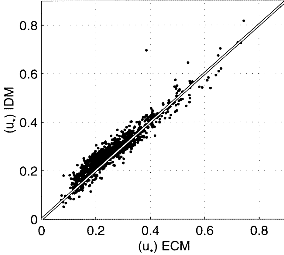
Figure 4. The friction velocity u_* [ \text{m s}^{-1} ] from ECM (x-axis) and IDM (y-axis).
