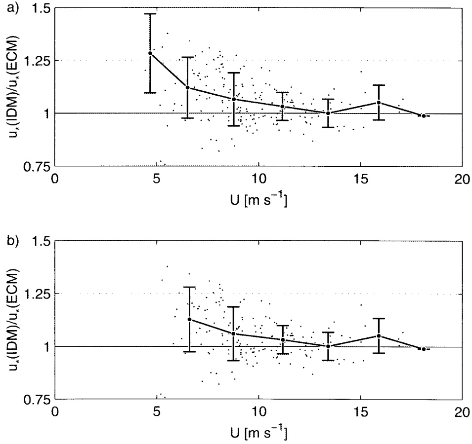
Figure 6. Ratio of u_* from IDM and u_* from ECM as a function of wind speed, symbols as in Figure 5: (a) All data, (b) only data with wave age 0.5 < c_0/(U_{10} \cos \theta) < 1.0 . Near-neutral data ( -0.02 < z/L < 0.02 ).
