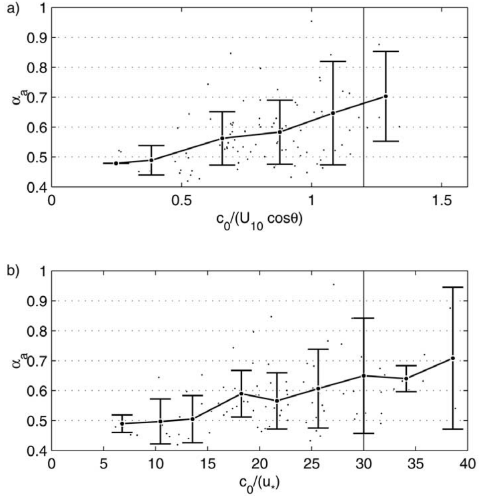
Figure 10. Effective values of the Kolmogorov constant, \alpha_a , as a function of wave age: (a) c_0/(U_{10} \cos \theta) , (b) c_0/u_* . Symbols as in Figure 5. Very near-neutral data ( -0.01 < z/L < 0.01 ).
