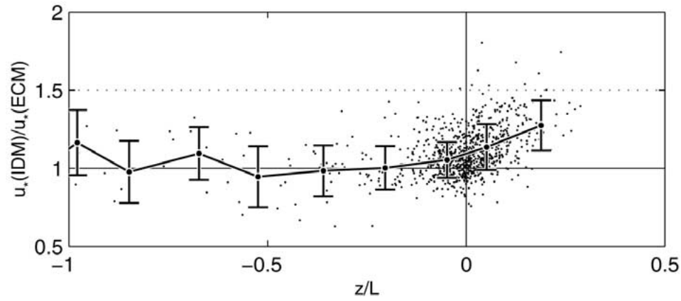
Figure 5. Ratio of u_* from IDM and u_* from ECM as a function of stability, z/L . The dots ( \cdot ) are the data, the solid line ( — ) the averaged curve, and the filled circles ( \bullet ) are the bin-averaged values with error bars.
