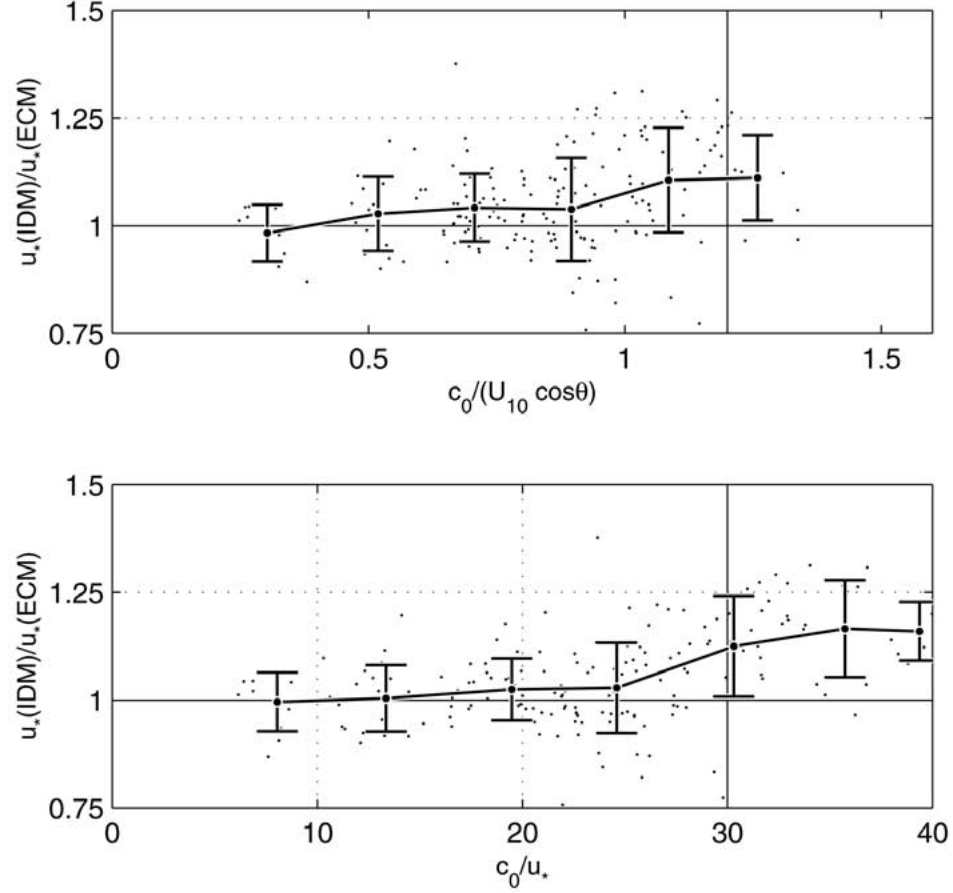
Figure 7. Ratio of u_* from IDM and u_* from ECM plotted as a function of two wave-age estimates: (a) as a function of c_0/(U_{10} \cos \theta) , (b) c_0/u_* . Symbols as in Figure 5. Near-neutral data ( -0.02 < z/L < 0.02 ).
