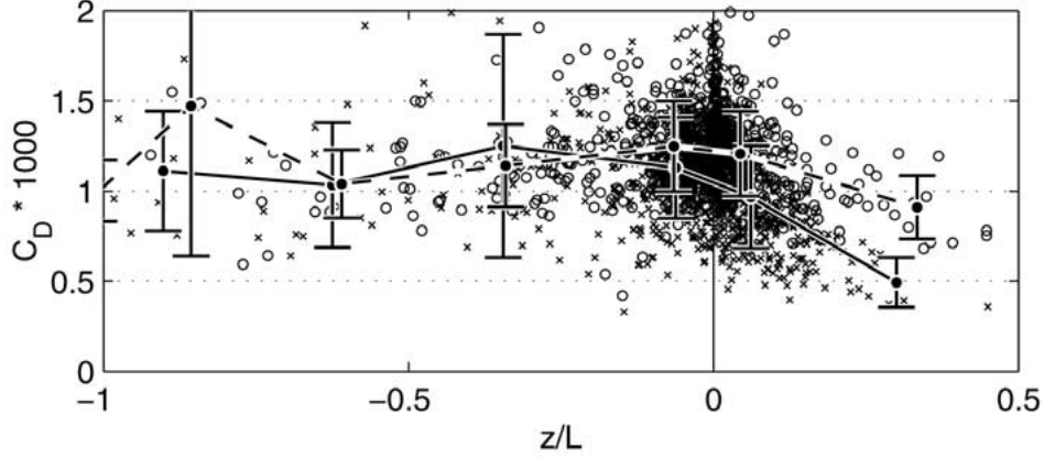
Figure 3. The drag coefficient as a function of the stability z/L , from the ECM, solid line (—), and IDM, dashed line (---). z/L has been determined with separate methods, as described in the text. Crosses ( \times ) are ECM and open circles ( \circ ) IDM. The filled circles ( \bullet ) show bin-averaged values with standard deviations.
