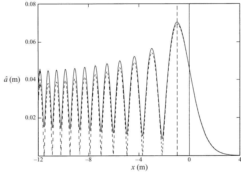
FIGURE 17. Variation of \hat{a} in the simulation of a straight caustic. The dashed line represents the absolute magnitude of \text{Ai}(-r) (the relation between r and x is given by (5.6a)) multiplied by a constant to make the resulting quantity equal to \hat{a} at the caustic x = 0 .
