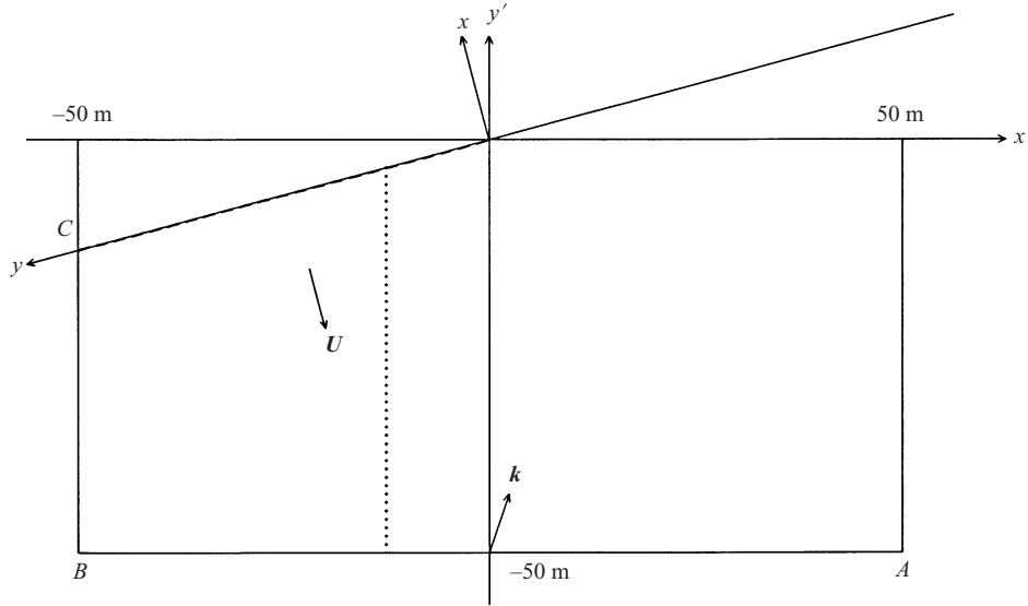
FIGURE 4. The domain of integration and the true ( y -axis) and predicted (dashed line) locations of the caustic in the simulation of a straight caustic.
