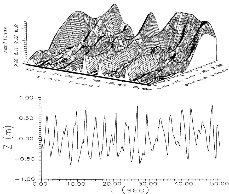
FIG. 4. The wavelet transform of field dataset 4. (a) Three-dimensional display of the modulus A(\tau, T) [with \zeta(\tau, T) \equiv A(\tau, T)e^{i\phi(\tau, T)} ], the period of the dominant waves being about 2.5 s; (b) the corresponding wave elevation \zeta(t) .
