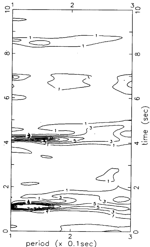
FIG. 7b. The isogram of I(\tau, T) .
