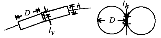
Fig. 3. Two floes frozen together on top of a wave field. The one on left is the side view and the one on right is the top view. The frozen area has a vertical dimension of l_v and horizontal dimension of l_h . Both floes can be composites of smaller floes formed at an earlier stage.
