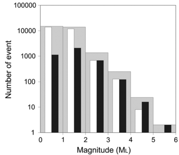
Fig. 5. Number of events reported by KIGAM's earthquake monitoring system versus magnitude. Gray, white and black bars represent number of events occurring during whole day, daytime and nighttime, respectively.
