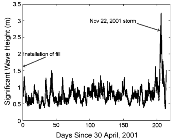
Fig. 5. Significant wave height at Torrey Pines Inner Buoy (20 m water depth) versus time.
