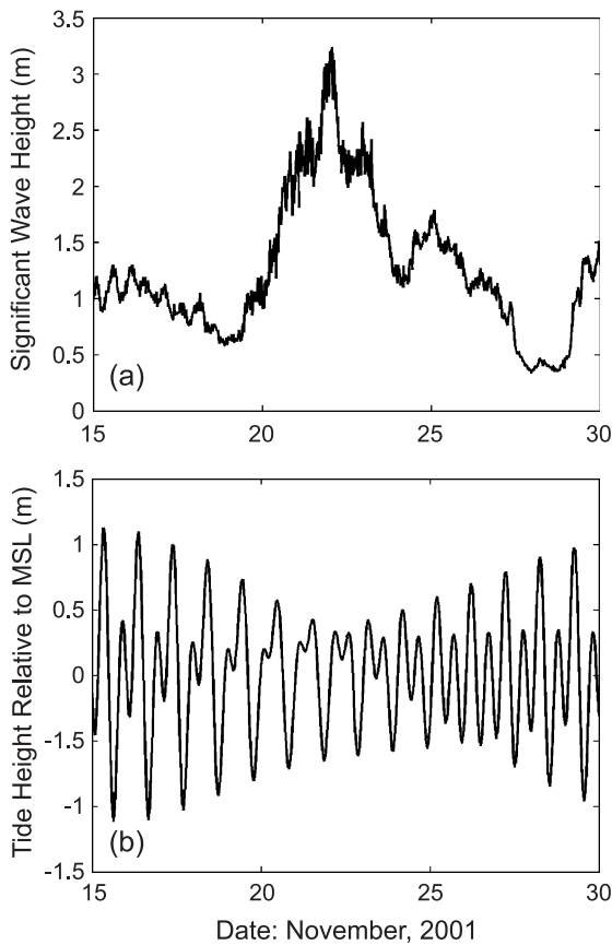
Fig. 7. (a) Significant wave height and (b) tidal elevation at Torrey Pines versus time.
