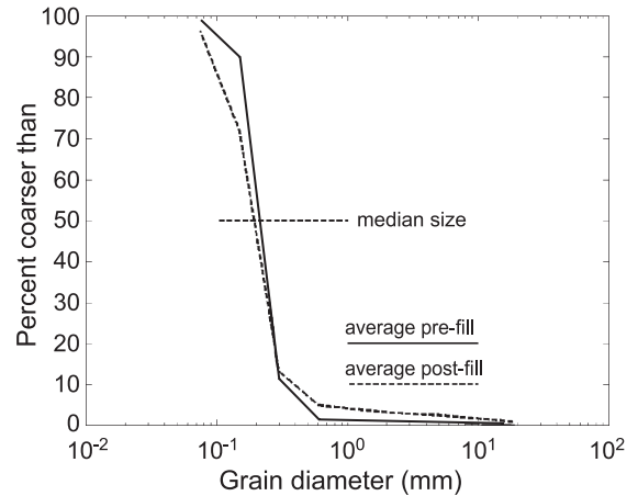
Fig. 3. Percent of sediment coarser than a size versus grain diameter.
