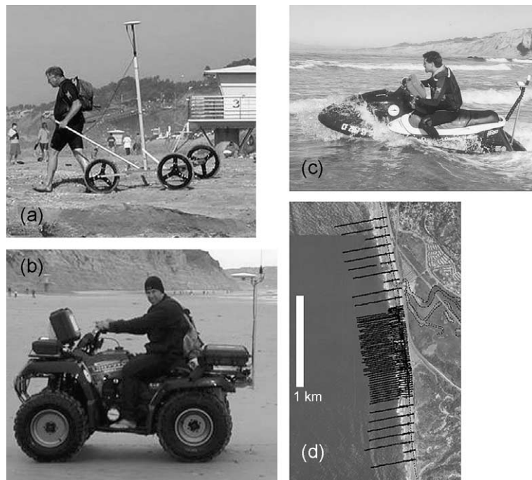
Fig. 4. GPS-equipped survey vehicles. (a) Cart, (b) all-terrain vehicle, (c) wave-runner and (d) typical survey vehicle tracks (black curves) superposed on an aerial photograph of the fill area and adjacent coastline.
