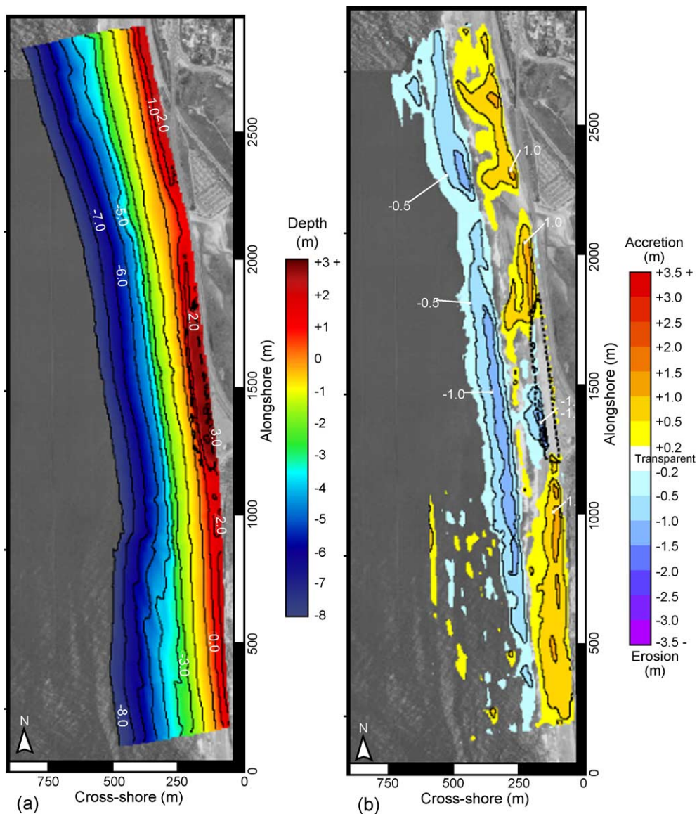
Fig. 6. (a) Bathymetry measured on 17 November 2001 along a 2700-m long strip centered on the initially nourished region (black dashed curves). Contours are depth in meters relative to MSL, and the contour interval is 1 m. (b) Changes in bathymetry between 27 April 2001 and 17 November 2001. The contour interval is 0.5 m. Changes less than 0.2 m are not shown. Color scales are to the right of each panel.
