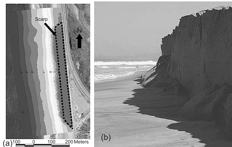
Fig. 2. (a) Configuration of the newly completed beach fill, 30 April 2001. Contours are depths relative to MSL. The elevated fill is indicated with a dashed curve. (b) Photograph of the seaward edge of the fill showing the 2-m high scarp.
