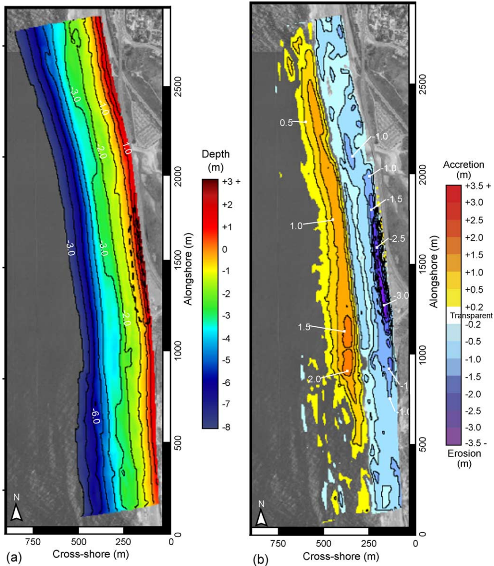
Fig. 9. (a) Bathymetry measured on 30 November 2001 (1 week after the storm) along a 2700-m long strip centered on the initially nourished region (black dashed curves). Contours are depth in meters relative to MSL, and the contour interval is 1 m. (b) Changes in bathymetry between 17 and 30 November 2001. Contour interval is 0.5 m. Format is similar to Fig. 6.
