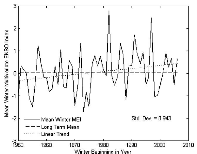
Figure 11. Long term variation in the mean winter season values of the Multivariate ENSO Index.
