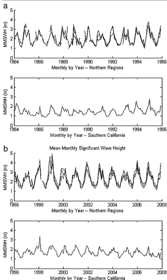
Figure 4. (a). MMSWH values for northern regions and Southern California, 1984–95. (b). MMSWH values for northern regions and Southern California, 1996–2008.
