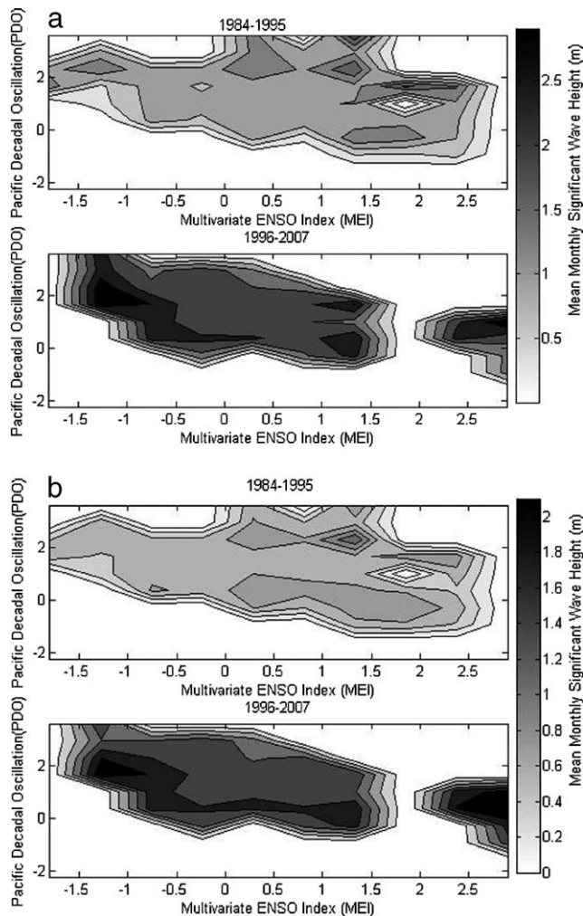
Figure 9. (a). Distribution of MMSWH means from the consolidated northern regions at coincident occurrences of MEI and PDO values over two periods. (b). Distribution of MMSWH means from the Southern California region at coincident occurrences of MEI and PDO values over two periods.
