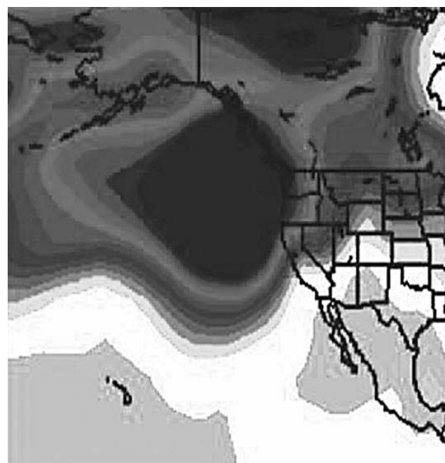
Figure 5. Gulf of Alaska low pressure area, December 16, 2002 (after Seymour, 2008).
