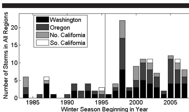
Figure 3. Occurrence by region of wave events with H_{m0} greater than 6 m for 24 hours (after Seymour, 2008).
