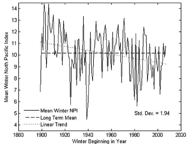
Figure 10. Long term variation in the mean winter season values of the North Pacific Index.
